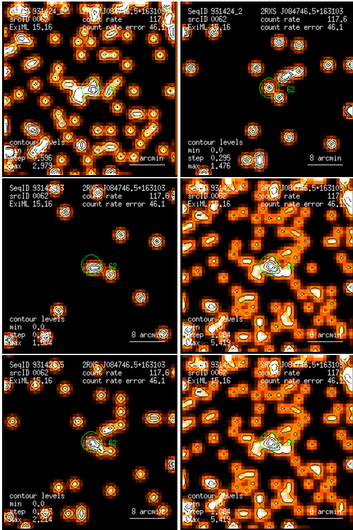
Figure 62: RASS 931424: detection 0062: band rate images, Gaussian filter: (1) PSPC channels 11 – 41, (2) 52 – 90, (3) 91 – 201, (4) 11 – 235, (5) 52 – 201, (6) 11 – 201. Broad band rates in counts/ks. Band rate contour levels in counts/ks/arcmin 2 .
