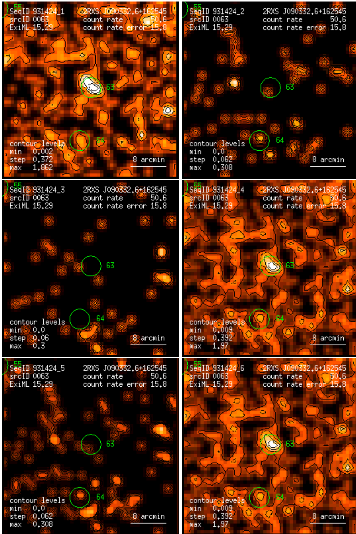
Figure 63: RASS 931424: detection 0063: band rate images, Gaussian filter: (1) PSPC channels 11 – 41, (2) 52 – 90, (3) 91 – 201, (4) 11 – 235, (5) 52 – 201, (6) 11 – 201. Broad band rates in counts/ks. Band rate contour levels in counts/ks/arcmin 2 .
