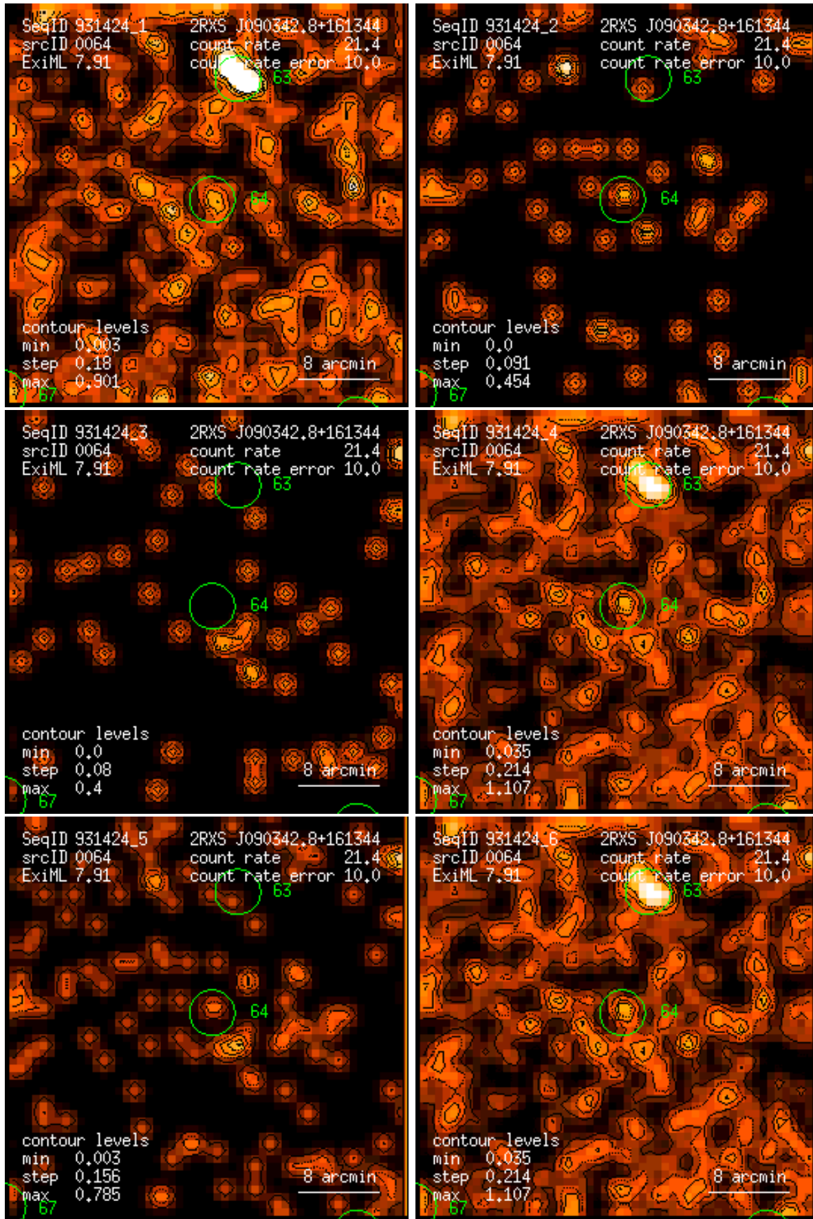
Figure 64: RASS 931424: detection 0064: band rate images, Gaussian filter: (1) PSPC channels 11 – 41, (2) 52 – 90, (3) 91 – 201, (4) 11 – 235, (5) 52 – 201, (6) 11 – 201. Broad band rates in counts/ks. Band rate contour levels in counts/ks/arcmin 2 .
