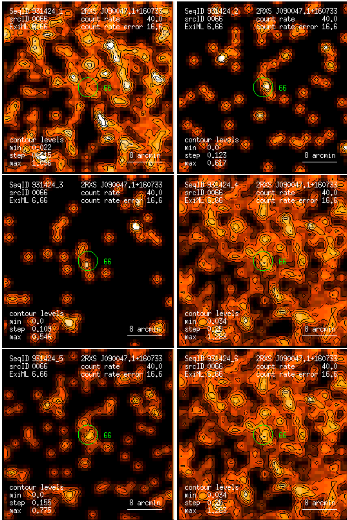
Figure 66: RASS 931424: detection 0066: band rate images, Gaussian filter: (1) PSPC channels 11 – 41, (2) 52 – 90, (3) 91 – 201, (4) 11 – 235, (5) 52 – 201, (6) 11 – 201. Broad band rates in counts/ks. Band rate contour levels in counts/ks/arcmin 2 .
