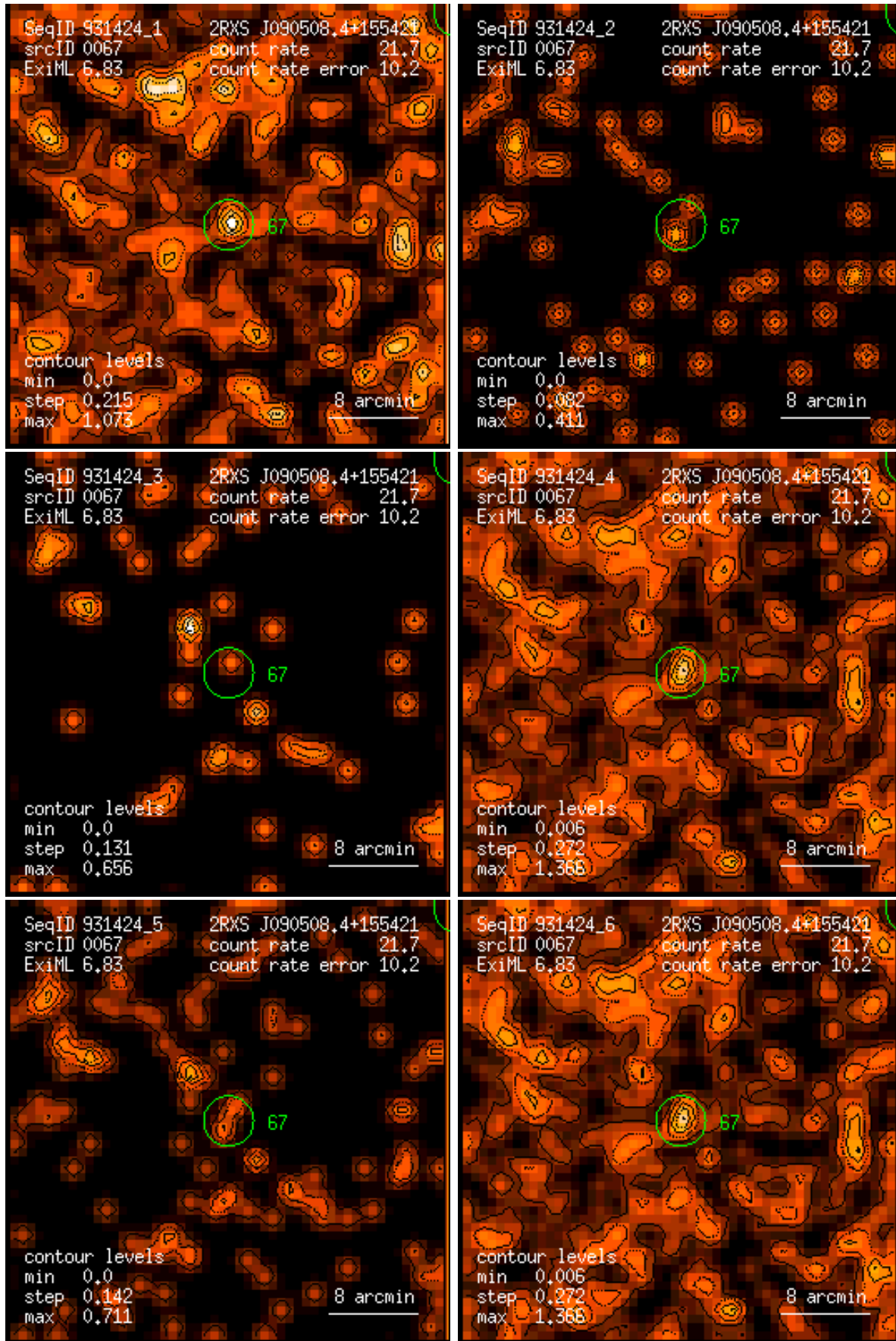
Figure 67: RASS 931424: detection 0067: band rate images, Gaussian filter: (1) PSPC channels 11 – 41, (2) 52 – 90, (3) 91 – 201, (4) 11 – 235, (5) 52 – 201, (6) 11 – 201. Broad band rates in counts/ks. Band rate contour levels in counts/ks/arcmin 2 .
