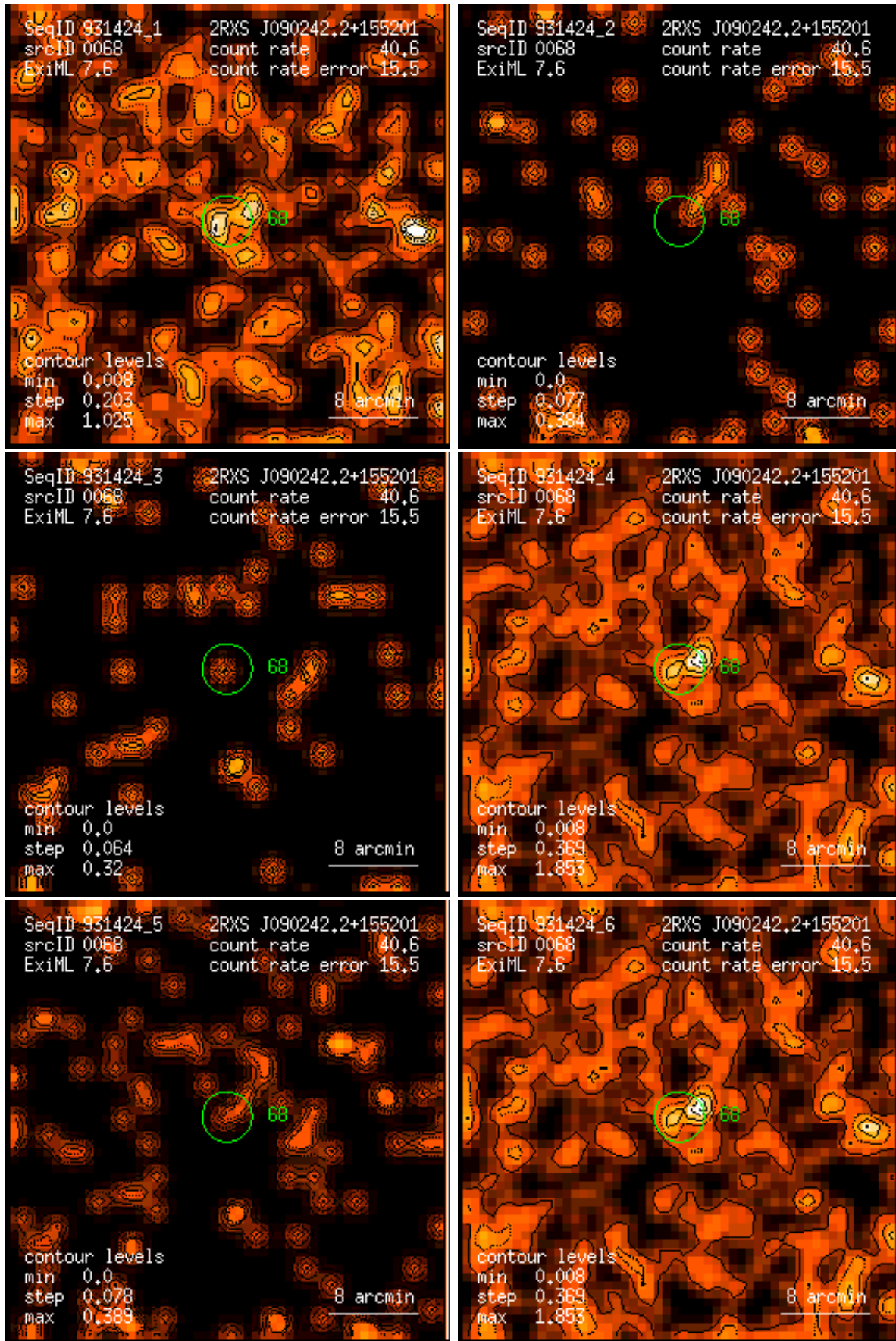
Figure 68: RASS 931424: detection 0068: band rate images, Gaussian filter: (1) PSPC channels 11 – 41, (2) 52 – 90, (3) 91 – 201, (4) 11 – 235, (5) 52 – 201, (6) 11 – 201. Broad band rates in counts/ks. Band rate contour levels in counts/ks/arcmin 2 .
