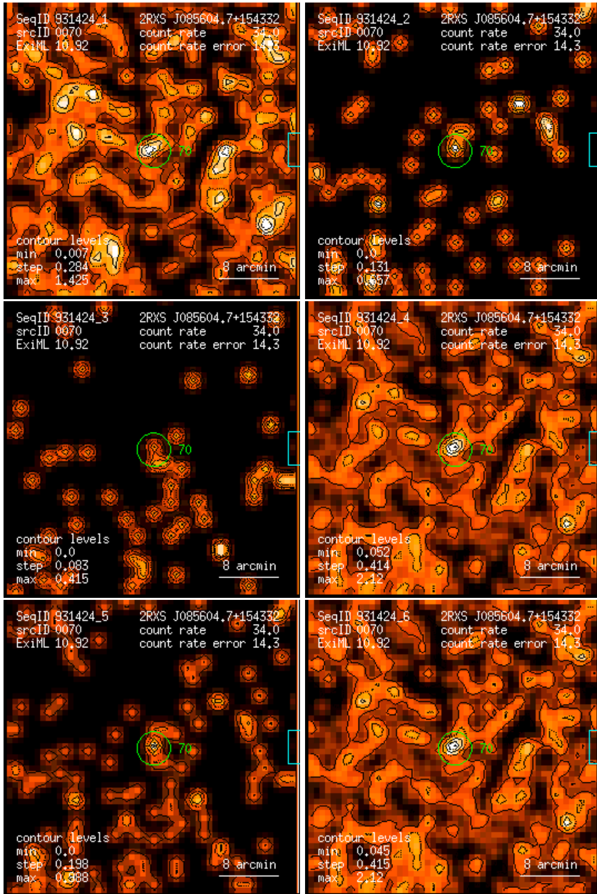
Figure 70: RASS 931424: detection 0070: band rate images, Gaussian filter: (1) PSPC channels 11 – 41, (2) 52 – 90, (3) 91 – 201, (4) 11 – 235, (5) 52 – 201, (6) 11 – 201. Broad band rates in counts/ks. Band rate contour levels in counts/ks/arcmin 2 .
