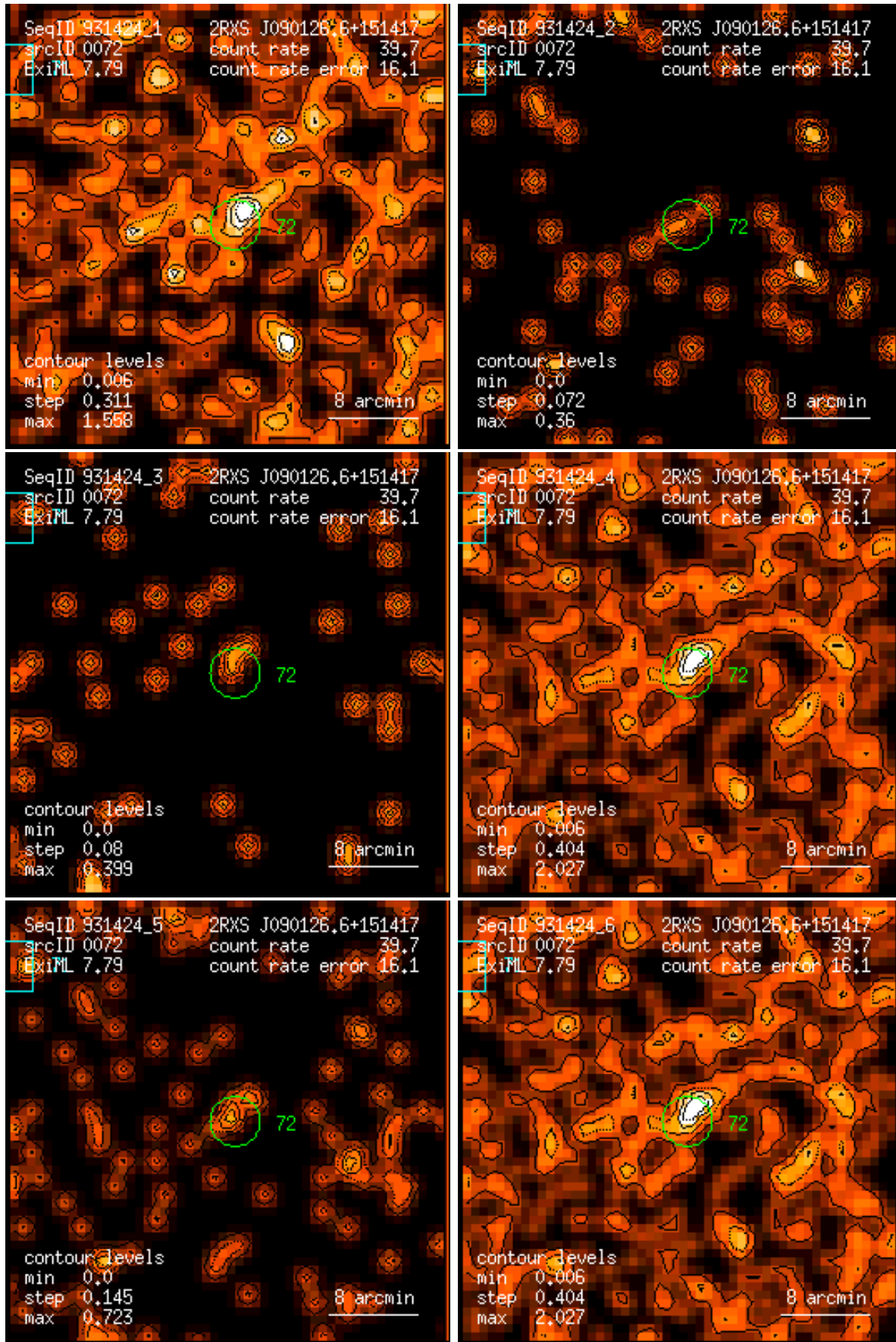
Figure 72: RASS 931424: detection 0072: band rate images, Gaussian filter: (1) PSPC channels 11 – 41, (2) 52 – 90, (3) 91 – 201, (4) 11 – 235, (5) 52 – 201, (6) 11 – 201. Broad band rates in counts/ks. Band rate contour levels in counts/ks/arcmin 2 .
