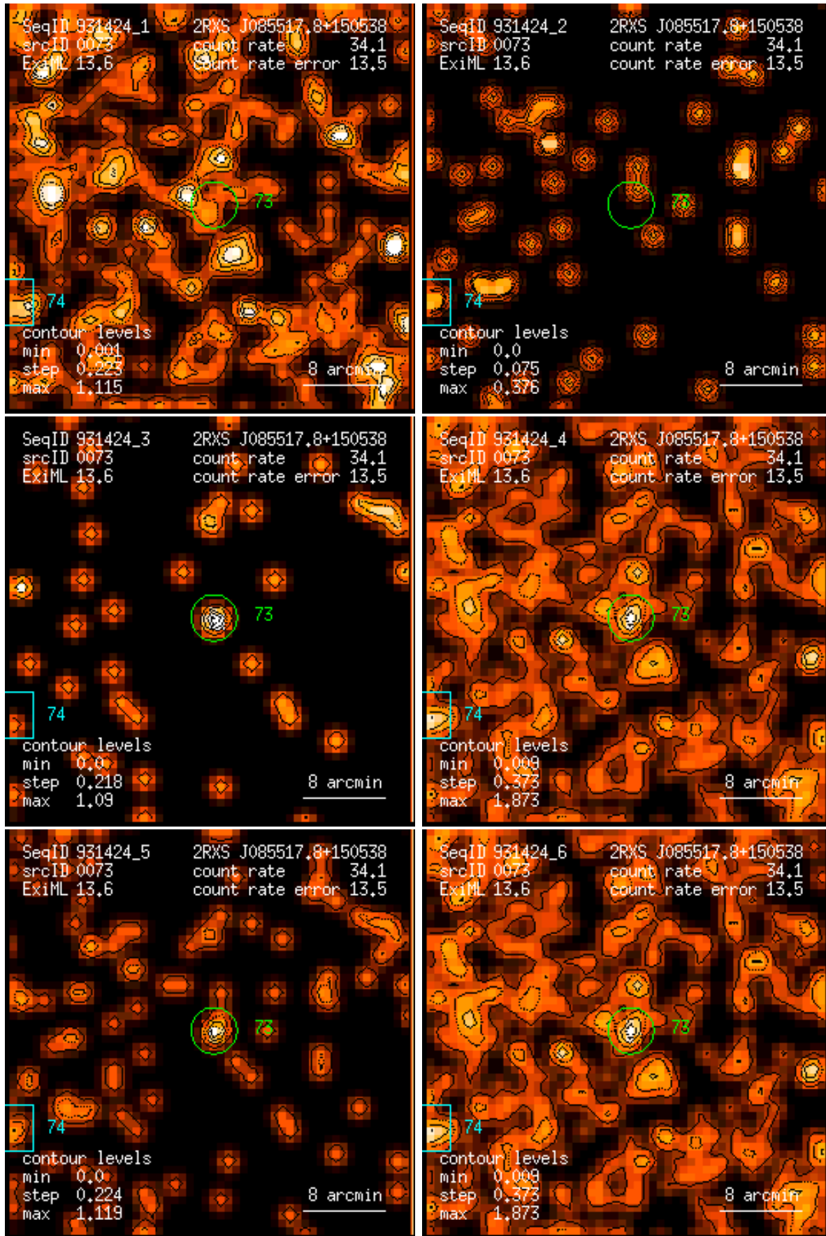
Figure 73: RASS 931424: detection 0073: band rate images, Gaussian filter: (1) PSPC channels 11 – 41, (2) 52 – 90, (3) 91 – 201, (4) 11 – 235, (5) 52 – 201, (6) 11 – 201. Broad band rates in counts/ks. Band rate contour levels in counts/ks/arcmin 2 .
