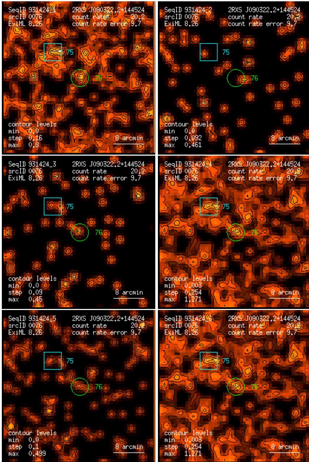
Figure 76: RASS 931424: detection 0076: band rate images, Gaussian filter: (1) PSPC channels 11 – 41, (2) 52 – 90, (3) 91 – 201, (4) 11 – 235, (5) 52 – 201, (6) 11 – 201. Broad band rates in counts/ks. Band rate contour levels in counts/ks/arcmin 2 .
