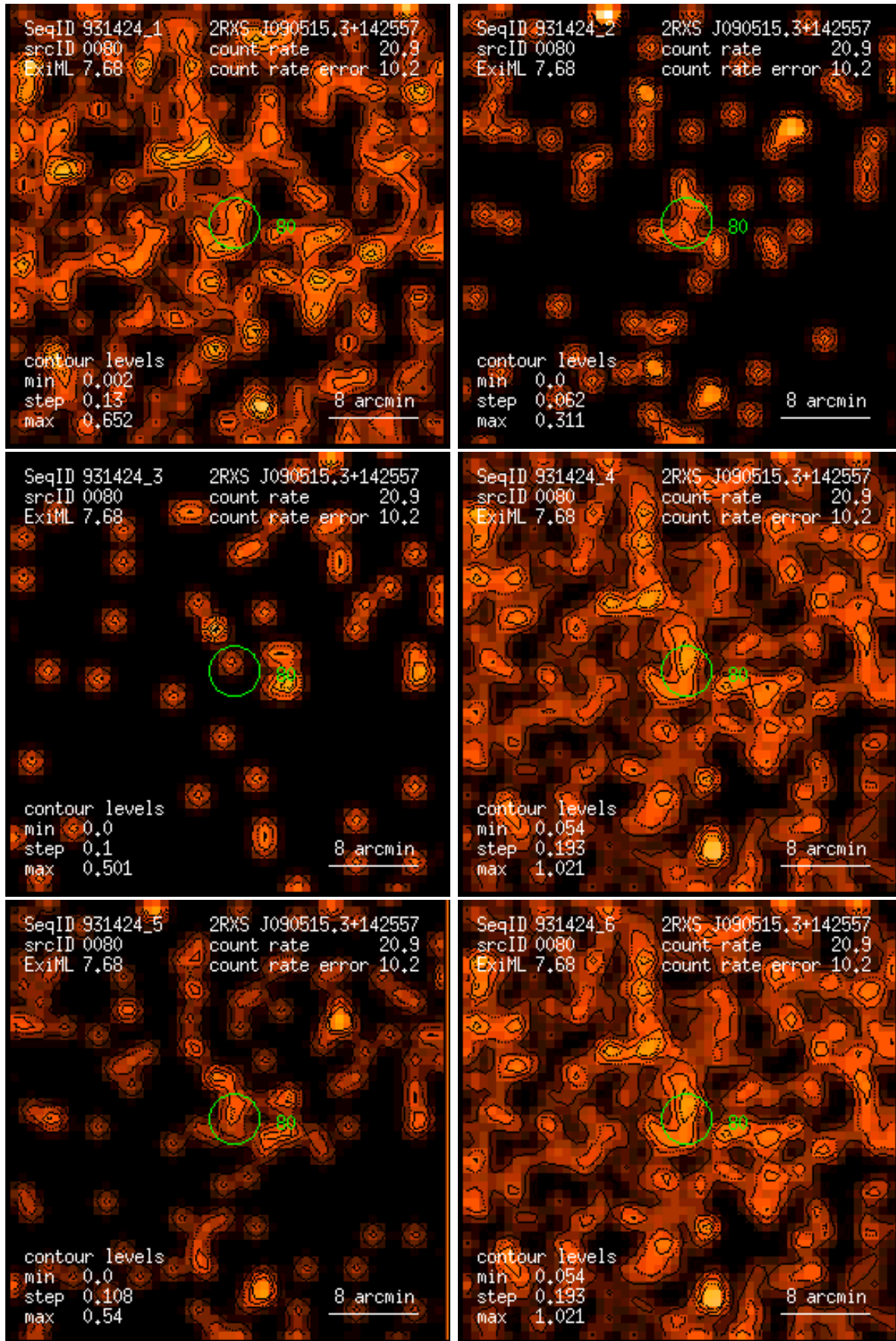
Figure 80: RASS 931424: detection 0080: band rate images, Gaussian filter: (1) PSPC channels 11 – 41, (2) 52 – 90, (3) 91 – 201, (4) 11 – 235, (5) 52 – 201, (6) 11 – 201. Broad band rates in counts/ks. Band rate contour levels in counts/ks/arcmin 2 .
