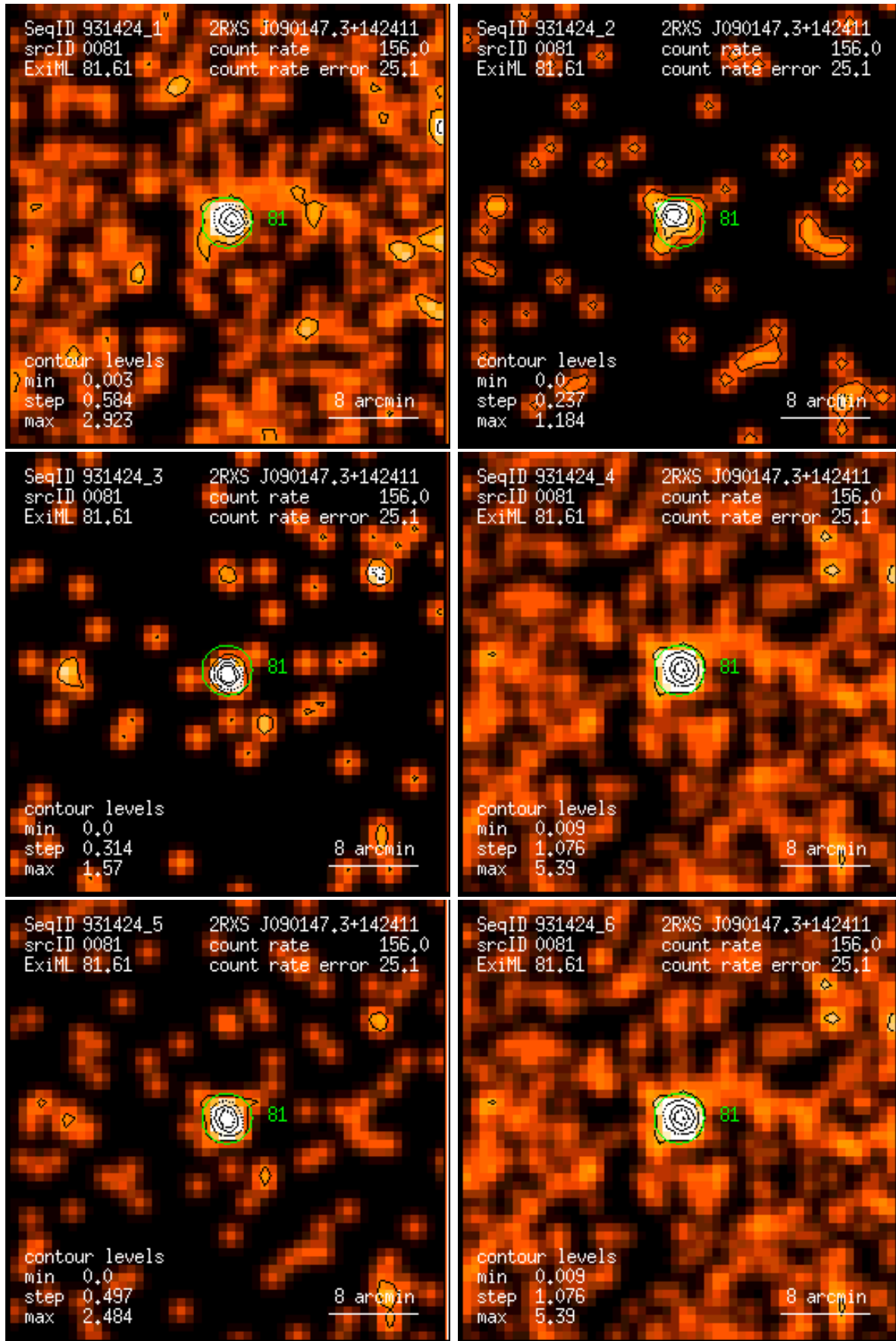
Figure 81: RASS 931424: detection 0081: band rate images, Gaussian filter: (1) PSPC channels 11 – 41, (2) 52 – 90, (3) 91 – 201, (4) 11 – 235, (5) 52 – 201, (6) 11 – 201. Broad band rates in counts/ks. Band rate contour levels in counts/ks/arcmin 2 .
