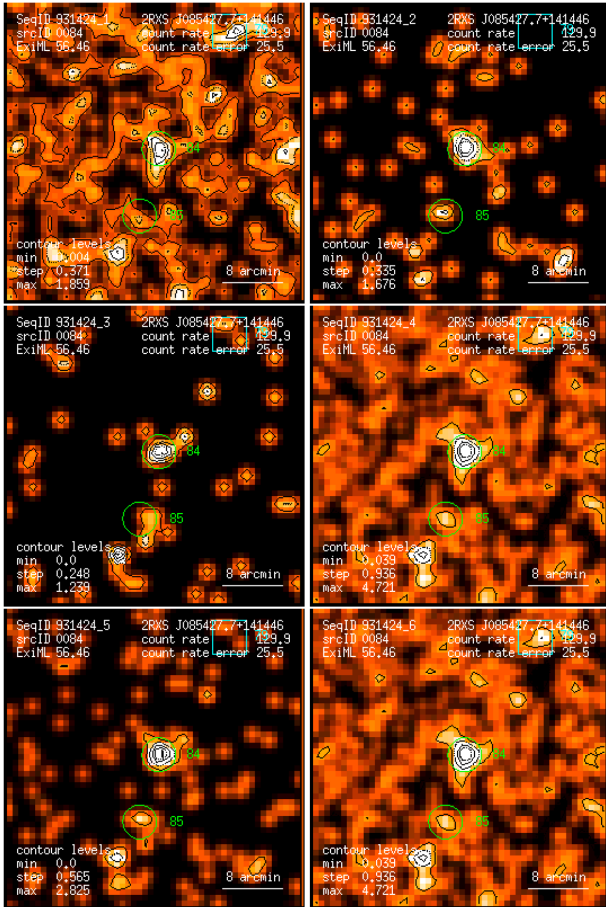
Figure 84: RASS 931424: detection 0084: band rate images, Gaussian filter: (1) PSPC channels 11 – 41, (2) 52 – 90, (3) 91 – 201, (4) 11 – 235, (5) 52 – 201, (6) 11 – 201. Broad band rates in counts/ks. Band rate contour levels in counts/ks/arcmin 2 .
