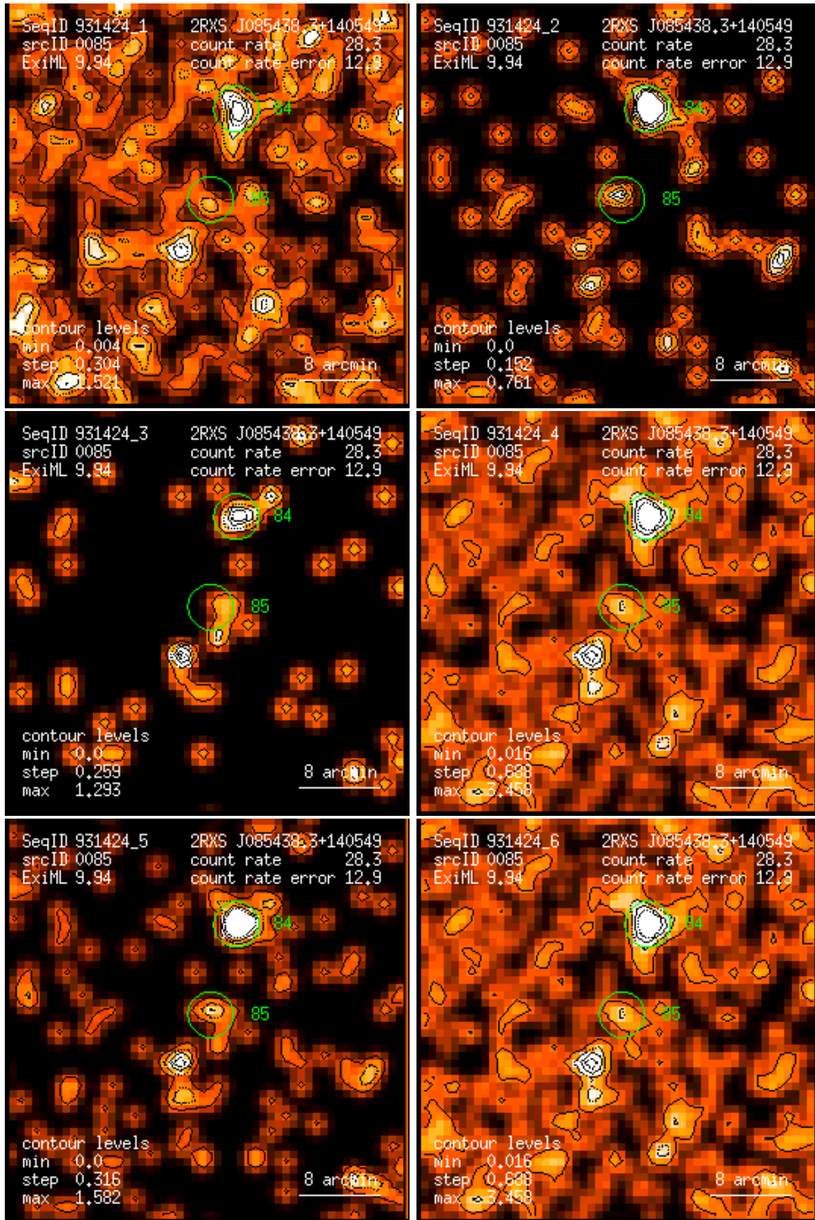
Figure 85: RASS 931424: detection 0085: band rate images, Gaussian filter: (1) PSPC channels 11 – 41, (2) 52 – 90, (3) 91 – 201, (4) 11 – 235, (5) 52 – 201, (6) 11 – 201. Broad band rates in counts/ks. Band rate contour levels in counts/ks/arcmin 2 .
