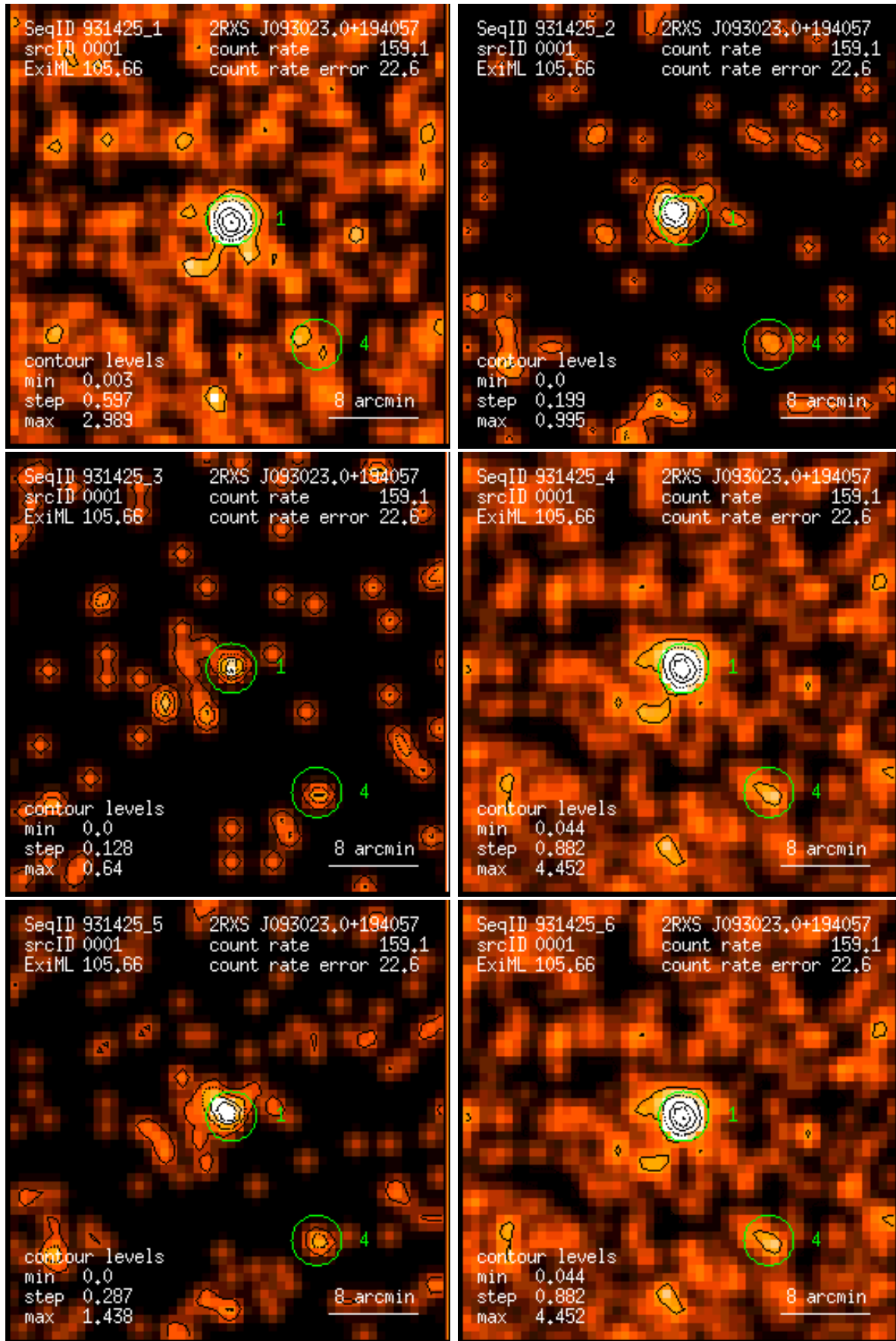
Figure 1: RASS 931425: detection 0001: band rate images, Gaussian filter: (1) PSPC channels 11 – 41, (2) 52 – 90, (3) 91 – 201, (4) 11 – 235, (5) 52 – 201, (6) 11 – 201. Broad band rates in counts/ks. Band rate contour levels in counts/ks/arcmin 2 .
