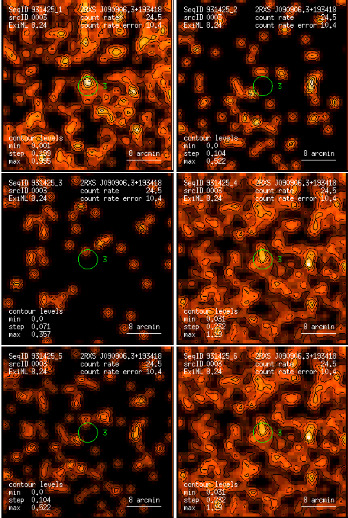
Figure 3: RASS 931425: detection 0003: band rate images, Gaussian filter: (1) PSPC channels 11 – 41, (2) 52 – 90, (3) 91 – 201, (4) 11 – 235, (5) 52 – 201, (6) 11 – 201. Broad band rates in counts/ks. Band rate contour levels in counts/ks/arcmin 2 .
