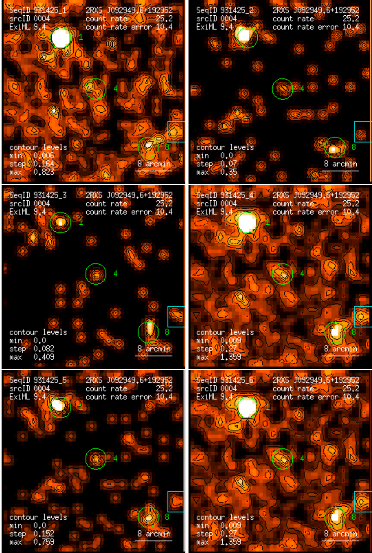
Figure 4: RASS 931425: detection 0004: band rate images, Gaussian filter: (1) PSPC channels 11 – 41, (2) 52 – 90, (3) 91 – 201, (4) 11 – 235, (5) 52 – 201, (6) 11 – 201. Broad band rates in counts/ks. Band rate contour levels in counts/ks/arcmin 2 .
