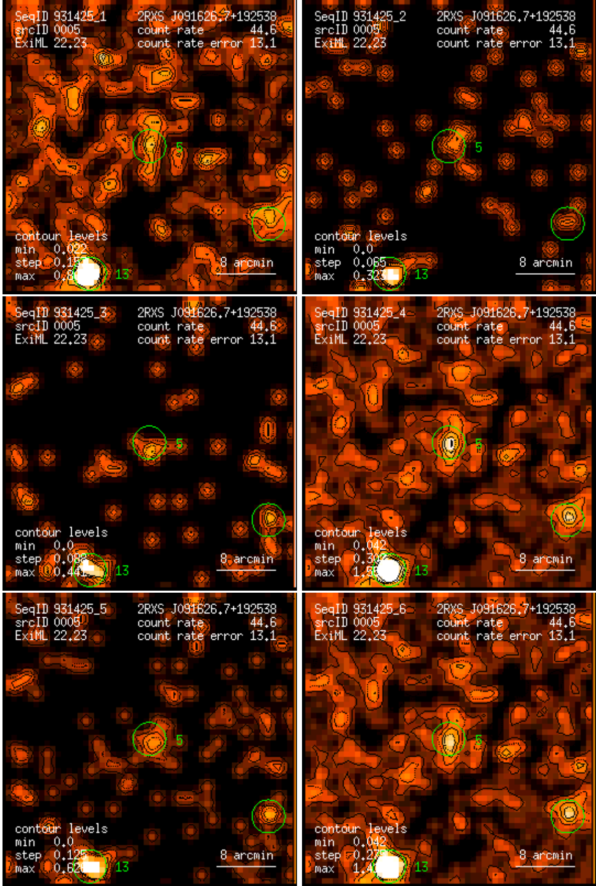
Figure 5: RASS 931425: detection 0005: band rate images, Gaussian filter: (1) PSPC channels 11 – 41, (2) 52 – 90, (3) 91 – 201, (4) 11 – 235, (5) 52 – 201, (6) 11 – 201. Broad band rates in counts/ks. Band rate contour levels in counts/ks/arcmin 2 .
