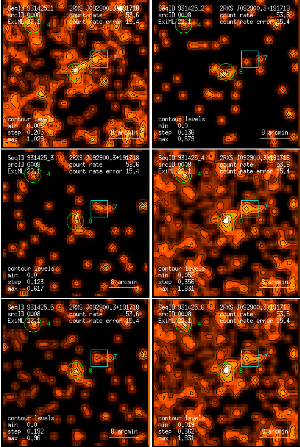
Figure 8: RASS 931425: detection 0008: band rate images, Gaussian filter: (1) PSPC channels 11 – 41, (2) 52 – 90, (3) 91 – 201, (4) 11 – 235, (5) 52 – 201, (6) 11 – 201. Broad band rates in counts/ks. Band rate contour levels in counts/ks/arcmin 2 .
