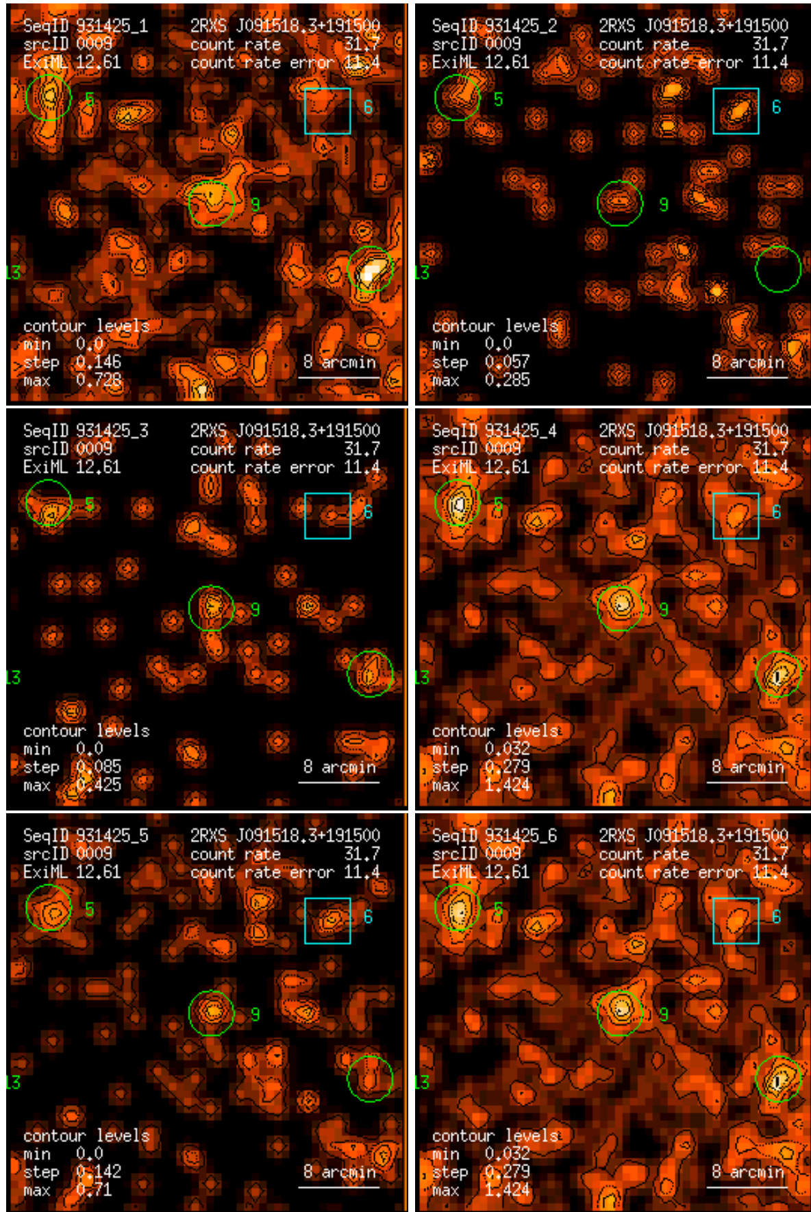
Figure 9: RASS 931425: detection 0009: band rate images, Gaussian filter: (1) PSPC channels 11 – 41, (2) 52 – 90, (3) 91 – 201, (4) 11 – 235, (5) 52 – 201, (6) 11 – 201. Broad band rates in counts/ks. Band rate contour levels in counts/ks/arcmin 2 .
