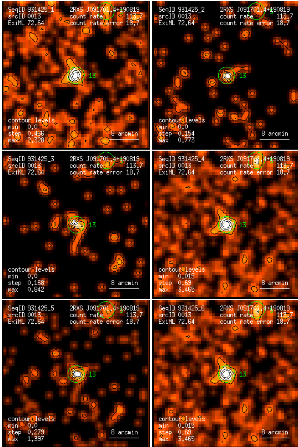
Figure 13: RASS 931425: detection 0013: band rate images, Gaussian filter: (1) PSPC channels 11 – 41, (2) 52 – 90, (3) 91 – 201, (4) 11 – 235, (5) 52 – 201, (6) 11 – 201. Broad band rates in counts/ks. Band rate contour levels in counts/ks/arcmin 2 .
