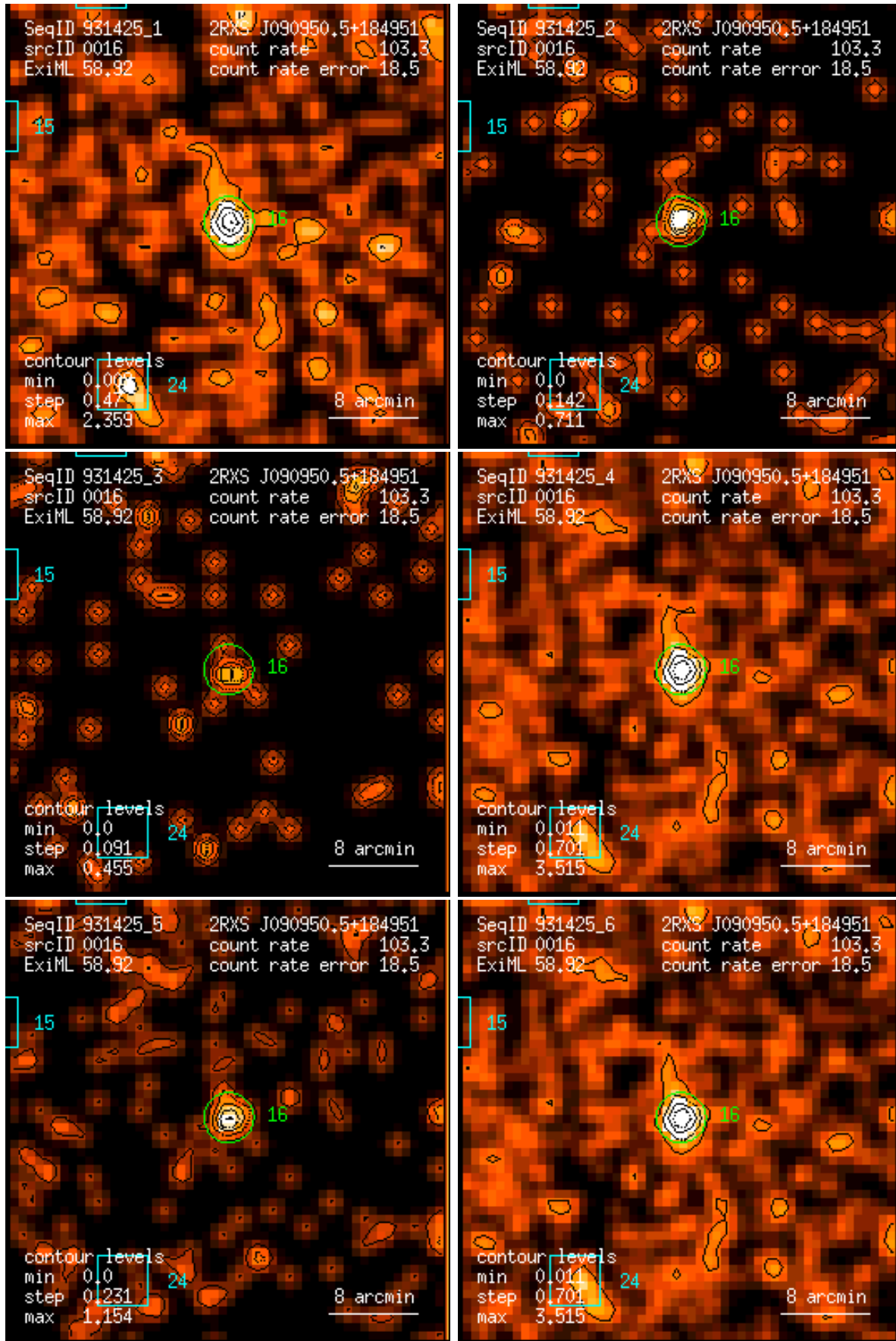
Figure 16: RASS 931425: detection 0016: band rate images, Gaussian filter: (1) PSPC channels 11 – 41, (2) 52 – 90, (3) 91 – 201, (4) 11 – 235, (5) 52 – 201, (6) 11 – 201. Broad band rates in counts/ks. Band rate contour levels in counts/ks/arcmin 2 .
