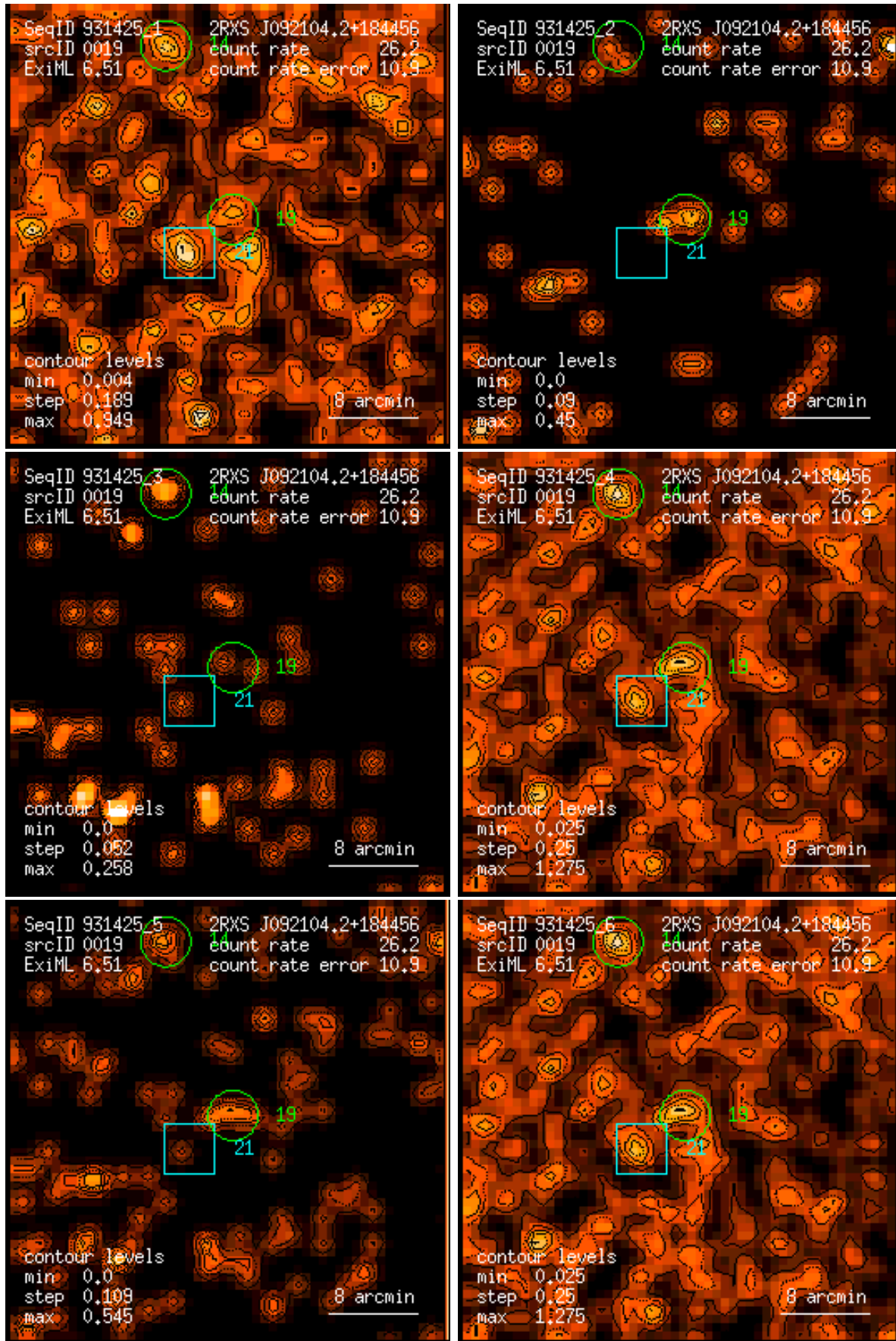
Figure 19: RASS 931425: detection 0019: band rate images, Gaussian filter: (1) PSPC channels 11 – 41, (2) 52 – 90, (3) 91 – 201, (4) 11 – 235, (5) 52 – 201, (6) 11 – 201. Broad band rates in counts/ks. Band rate contour levels in counts/ks/arcmin 2 .
