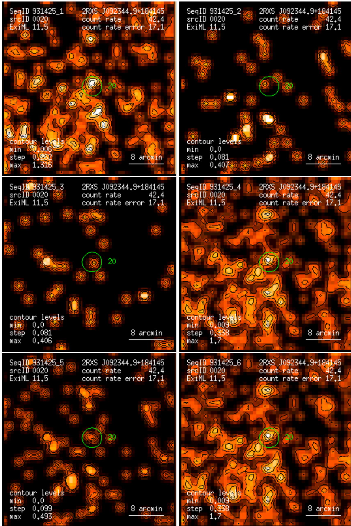
Figure 20: RASS 931425: detection 0020: band rate images, Gaussian filter: (1) PSPC channels 11 – 41, (2) 52 – 90, (3) 91 – 201, (4) 11 – 235, (5) 52 – 201, (6) 11 – 201. Broad band rates in counts/ks. Band rate contour levels in counts/ks/arcmin 2 .
