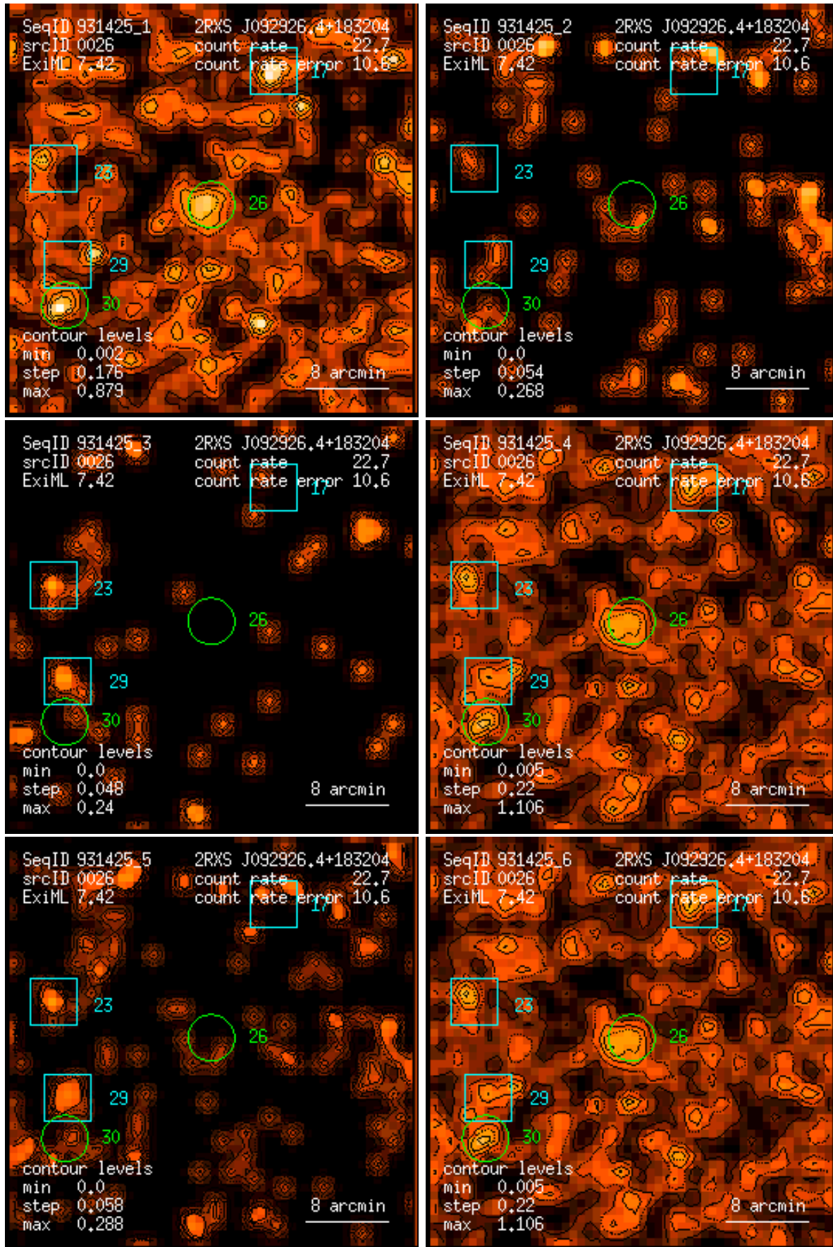
Figure 26: RASS 931425: detection 0026: band rate images, Gaussian filter: (1) PSPC channels 11 – 41, (2) 52 – 90, (3) 91 – 201, (4) 11 – 235, (5) 52 – 201, (6) 11 – 201. Broad band rates in counts/ks. Band rate contour levels in counts/ks/arcmin 2 .
