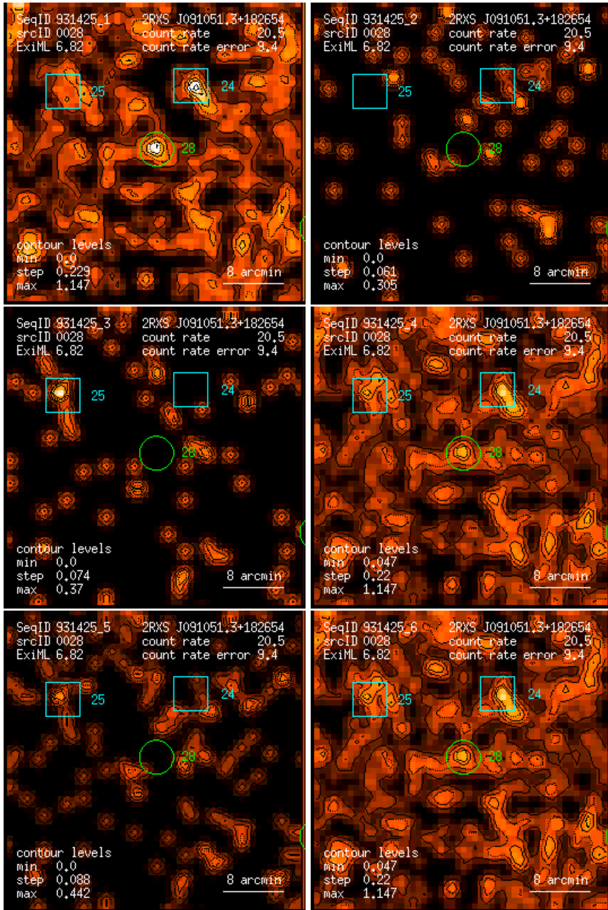
Figure 28: RASS 931425: detection 0028: band rate images, Gaussian filter: (1) PSPC channels 11 – 41, (2) 52 – 90, (3) 91 – 201, (4) 11 – 235, (5) 52 – 201, (6) 11 – 201. Broad band rates in counts/ks. Band rate contour levels in counts/ks/arcmin 2 .
