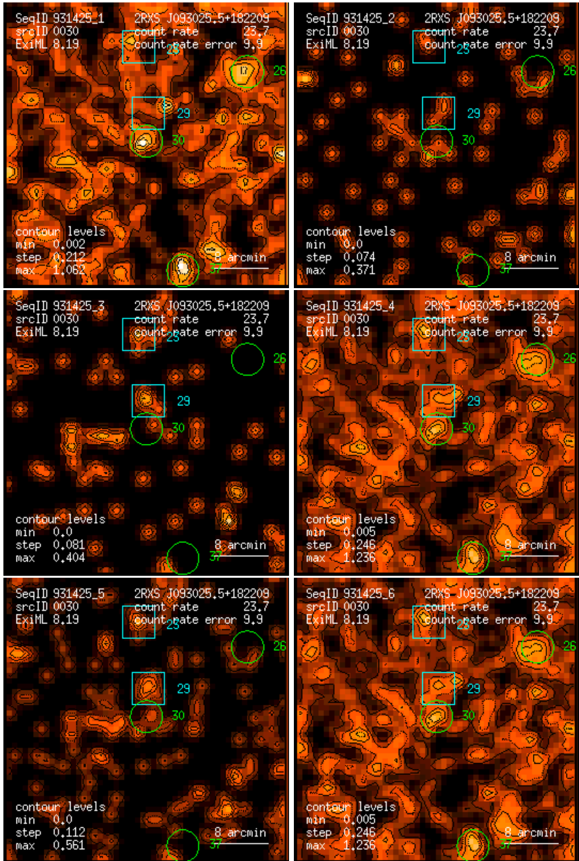
Figure 30: RASS 931425: detection 0030: band rate images, Gaussian filter: (1) PSPC channels 11 – 41, (2) 52 – 90, (3) 91 – 201, (4) 11 – 235, (5) 52 – 201, (6) 11 – 201. Broad band rates in counts/ks. Band rate contour levels in counts/ks/arcmin 2 .
