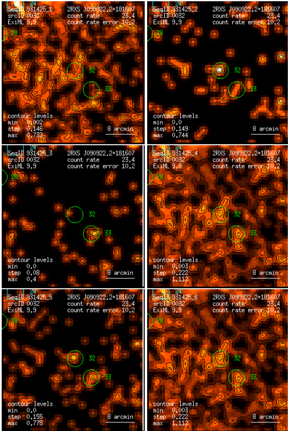
Figure 32: RASS 931425: detection 0032: band rate images, Gaussian filter: (1) PSPC channels 11 – 41, (2) 52 – 90, (3) 91 – 201, (4) 11 – 235, (5) 52 – 201, (6) 11 – 201. Broad band rates in counts/ks. Band rate contour levels in counts/ks/arcmin 2 .
