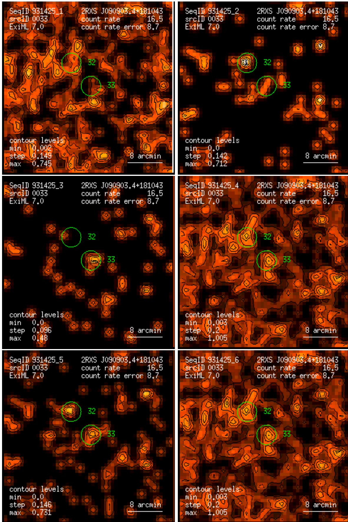
Figure 33: RASS 931425: detection 0033: band rate images, Gaussian filter: (1) PSPC channels 11 – 41, (2) 52 – 90, (3) 91 – 201, (4) 11 – 235, (5) 52 – 201, (6) 11 – 201. Broad band rates in counts/ks. Band rate contour levels in counts/ks/arcmin 2 .
