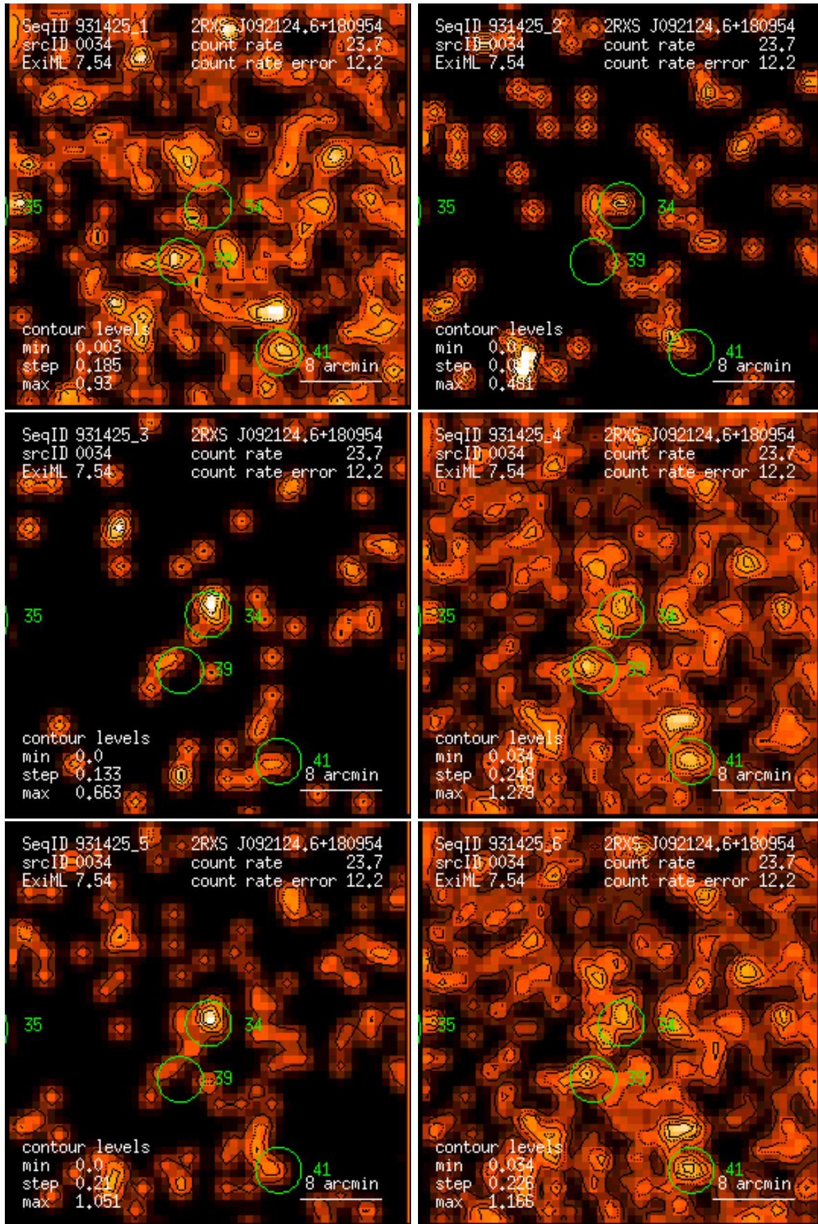
Figure 34: RASS 931425: detection 0034: band rate images, Gaussian filter: (1) PSPC channels 11 – 41, (2) 52 – 90, (3) 91 – 201, (4) 11 – 235, (5) 52 – 201, (6) 11 – 201. Broad band rates in counts/ks. Band rate contour levels in counts/ks/arcmin 2 .
