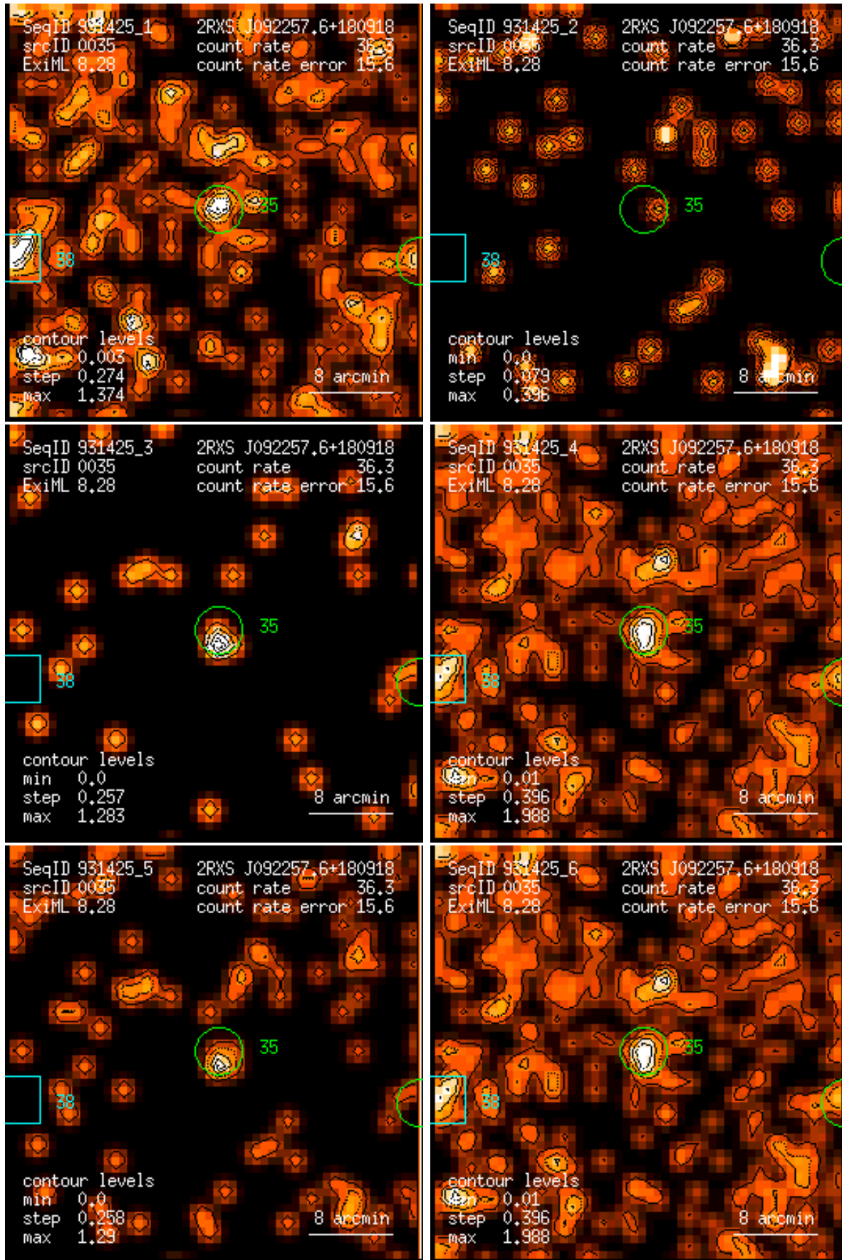
Figure 35: RASS 931425: detection 0035: band rate images, Gaussian filter: (1) PSPC channels 11 – 41, (2) 52 – 90, (3) 91 – 201, (4) 11 – 235, (5) 52 – 201, (6) 11 – 201. Broad band rates in counts/ks. Band rate contour levels in counts/ks/arcmin 2 .
