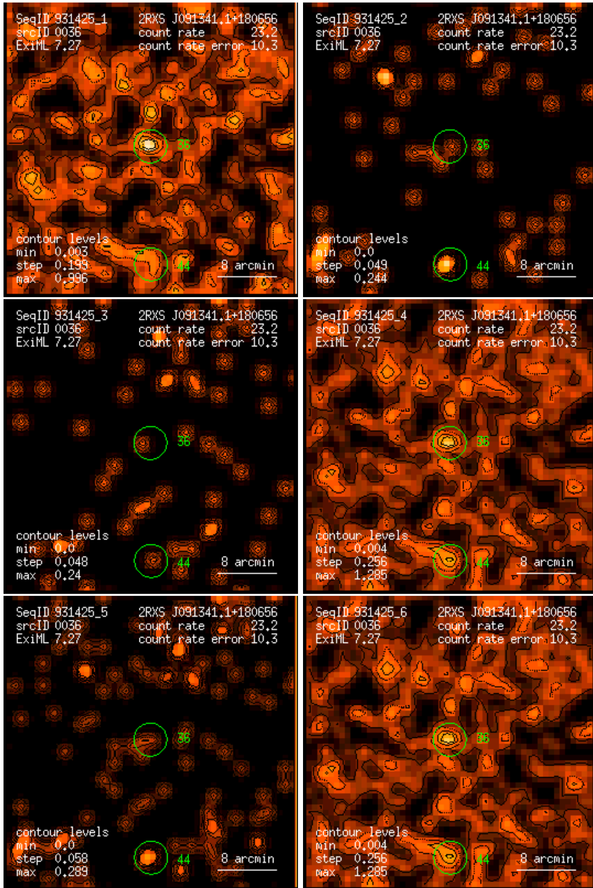
Figure 36: RASS 931425: detection 0036: band rate images, Gaussian filter: (1) PSPC channels 11 – 41, (2) 52 – 90, (3) 91 – 201, (4) 11 – 235, (5) 52 – 201, (6) 11 – 201. Broad band rates in counts/ks. Band rate contour levels in counts/ks/arcmin 2 .
