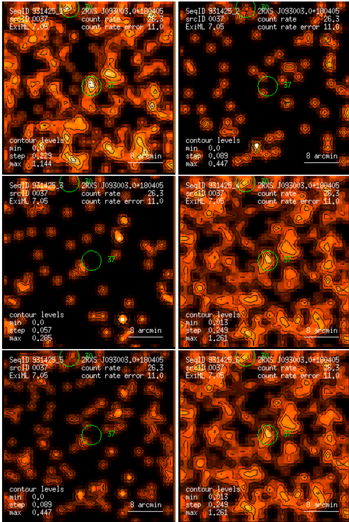
Figure 37: RASS 931425: detection 0037: band rate images, Gaussian filter: (1) PSPC channels 11 – 41, (2) 52 – 90, (3) 91 – 201, (4) 11 – 235, (5) 52 – 201, (6) 11 – 201. Broad band rates in counts/ks. Band rate contour levels in counts/ks/arcmin 2 .
