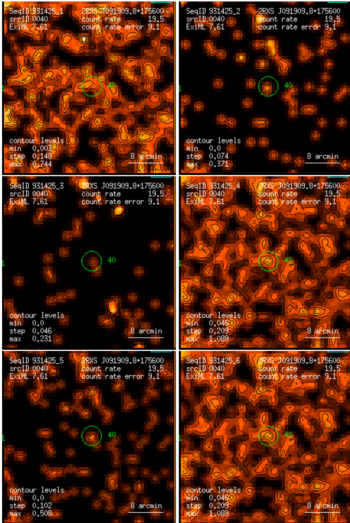
Figure 40: RASS 931425: detection 0040: band rate images, Gaussian filter: (1) PSPC channels 11 – 41, (2) 52 – 90, (3) 91 – 201, (4) 11 – 235, (5) 52 – 201, (6) 11 – 201. Broad band rates in counts/ks. Band rate contour levels in counts/ks/arcmin 2 .
