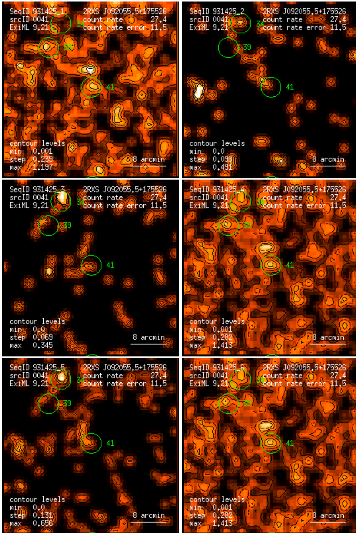
Figure 41: RASS 931425: detection 0041: band rate images, Gaussian filter: (1) PSPC channels 11 – 41, (2) 52 – 90, (3) 91 – 201, (4) 11 – 235, (5) 52 – 201, (6) 11 – 201. Broad band rates in counts/ks. Band rate contour levels in counts/ks/arcmin 2 .
