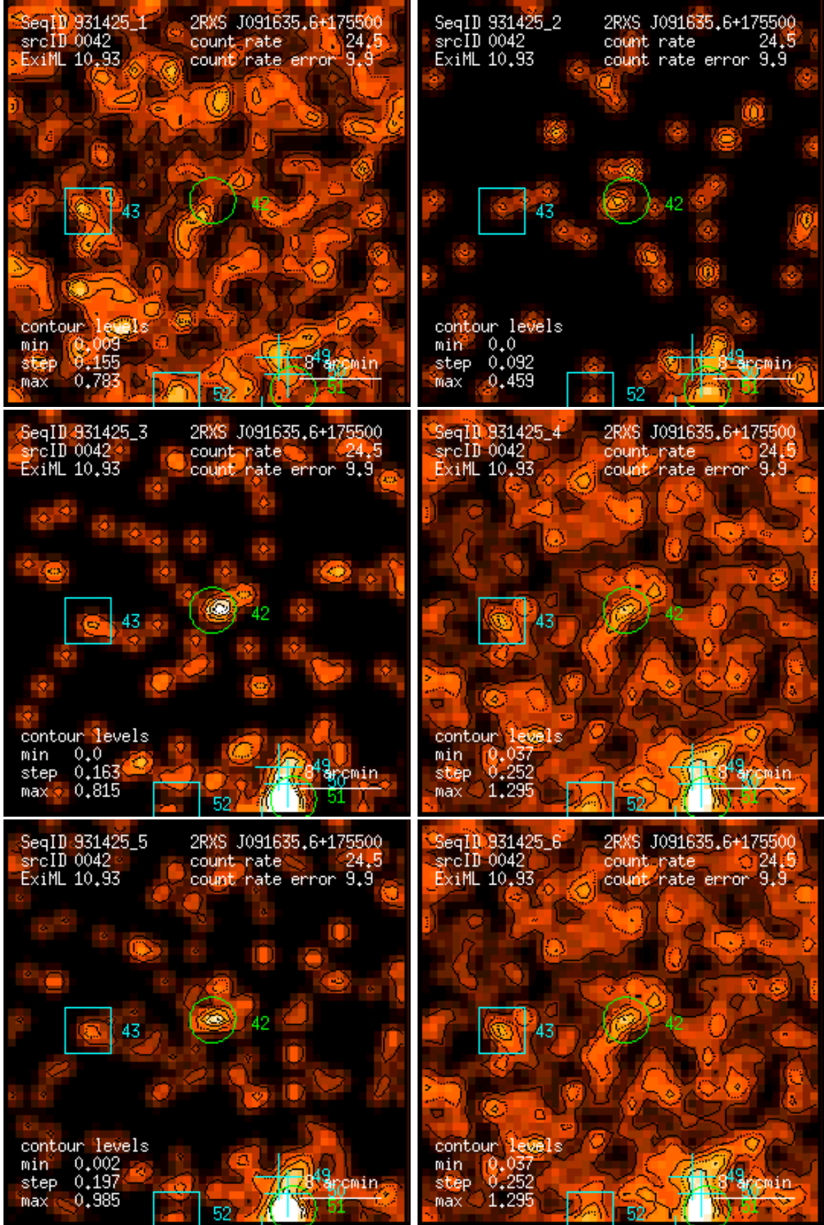
Figure 42: RASS 931425: detection 0042: band rate images, Gaussian filter: (1) PSPC channels 11 – 41, (2) 52 – 90, (3) 91 – 201, (4) 11 – 235, (5) 52 – 201, (6) 11 – 201. Broad band rates in counts/ks. Band rate contour levels in counts/ks/arcmin 2 .
