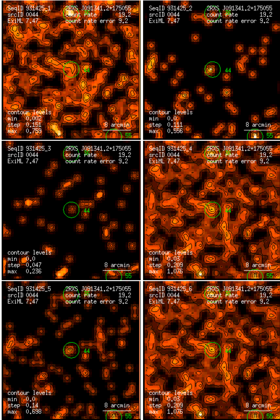
Figure 44: RASS 931425: detection 0044: band rate images, Gaussian filter: (1) PSPC channels 11 – 41, (2) 52 – 90, (3) 91 – 201, (4) 11 – 235, (5) 52 – 201, (6) 11 – 201. Broad band rates in counts/ks. Band rate contour levels in counts/ks/arcmin 2 .
