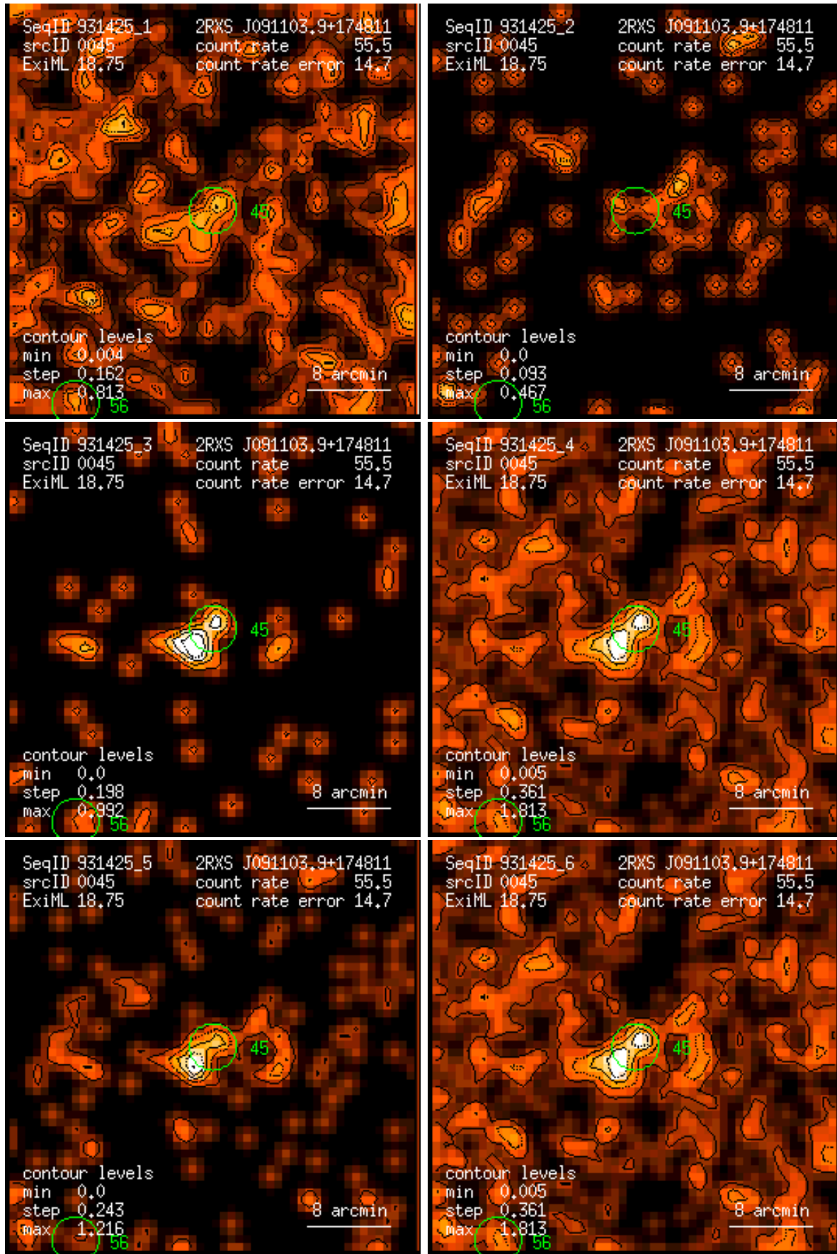
Figure 45: RASS 931425: detection 0045: band rate images, Gaussian filter: (1) PSPC channels 11 – 41, (2) 52 – 90, (3) 91 – 201, (4) 11 – 235, (5) 52 – 201, (6) 11 – 201. Broad band rates in counts/ks. Band rate contour levels in counts/ks/arcmin 2 .
