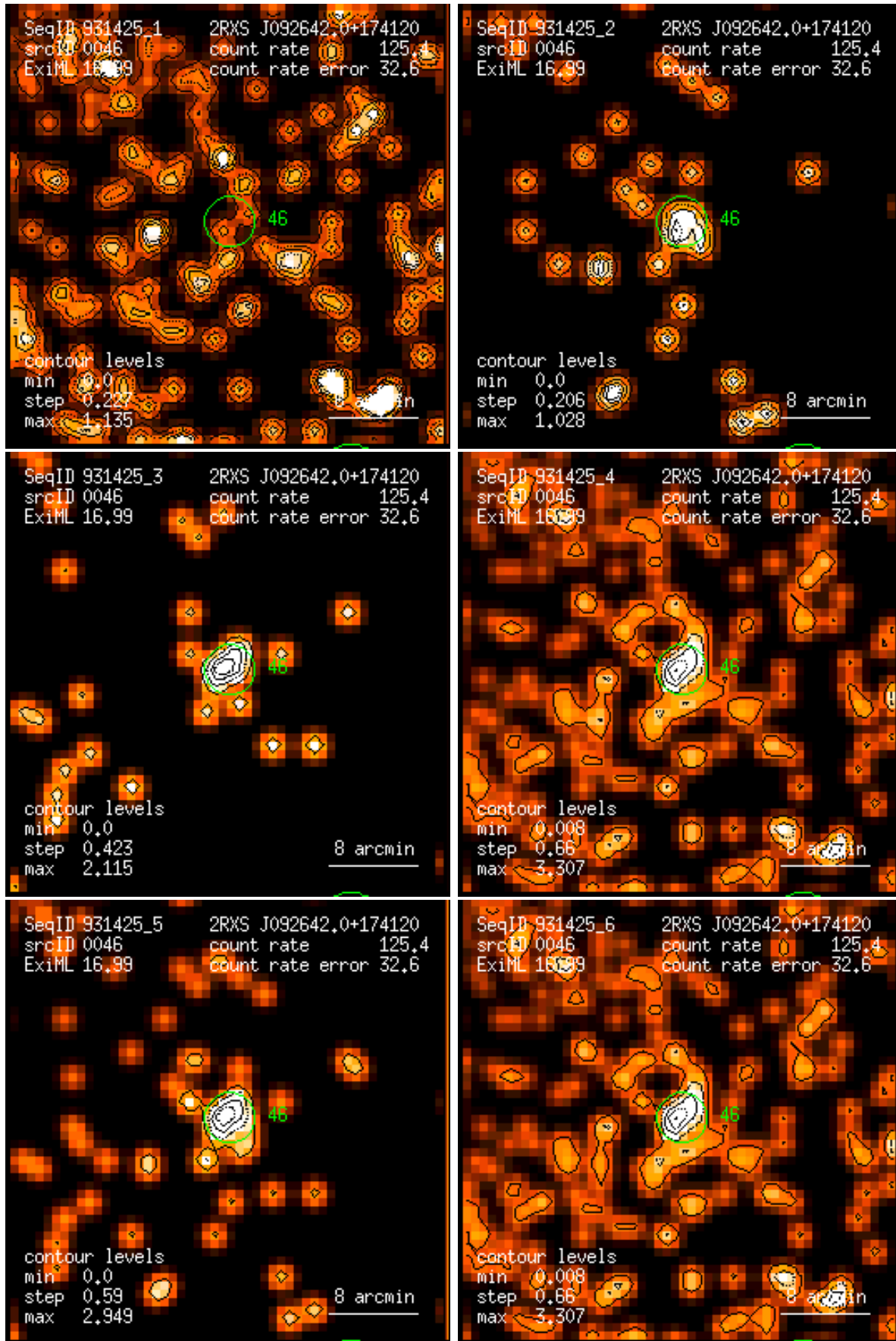
Figure 46: RASS 931425: detection 0046: band rate images, Gaussian filter: (1) PSPC channels 11 – 41, (2) 52 – 90, (3) 91 – 201, (4) 11 – 235, (5) 52 – 201, (6) 11 – 201. Broad band rates in counts/ks. Band rate contour levels in counts/ks/arcmin 2 .
