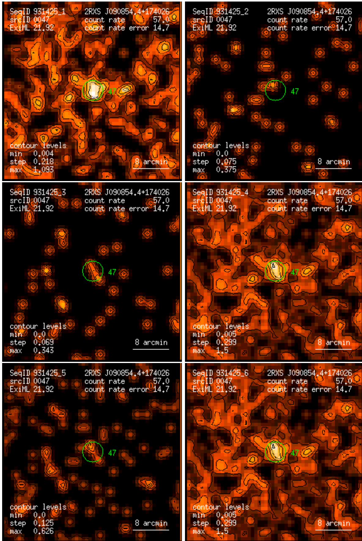
Figure 47: RASS 931425: detection 0047: band rate images, Gaussian filter: (1) PSPC channels 11 – 41, (2) 52 – 90, (3) 91 – 201, (4) 11 – 235, (5) 52 – 201, (6) 11 – 201. Broad band rates in counts/ks. Band rate contour levels in counts/ks/arcmin 2 .
