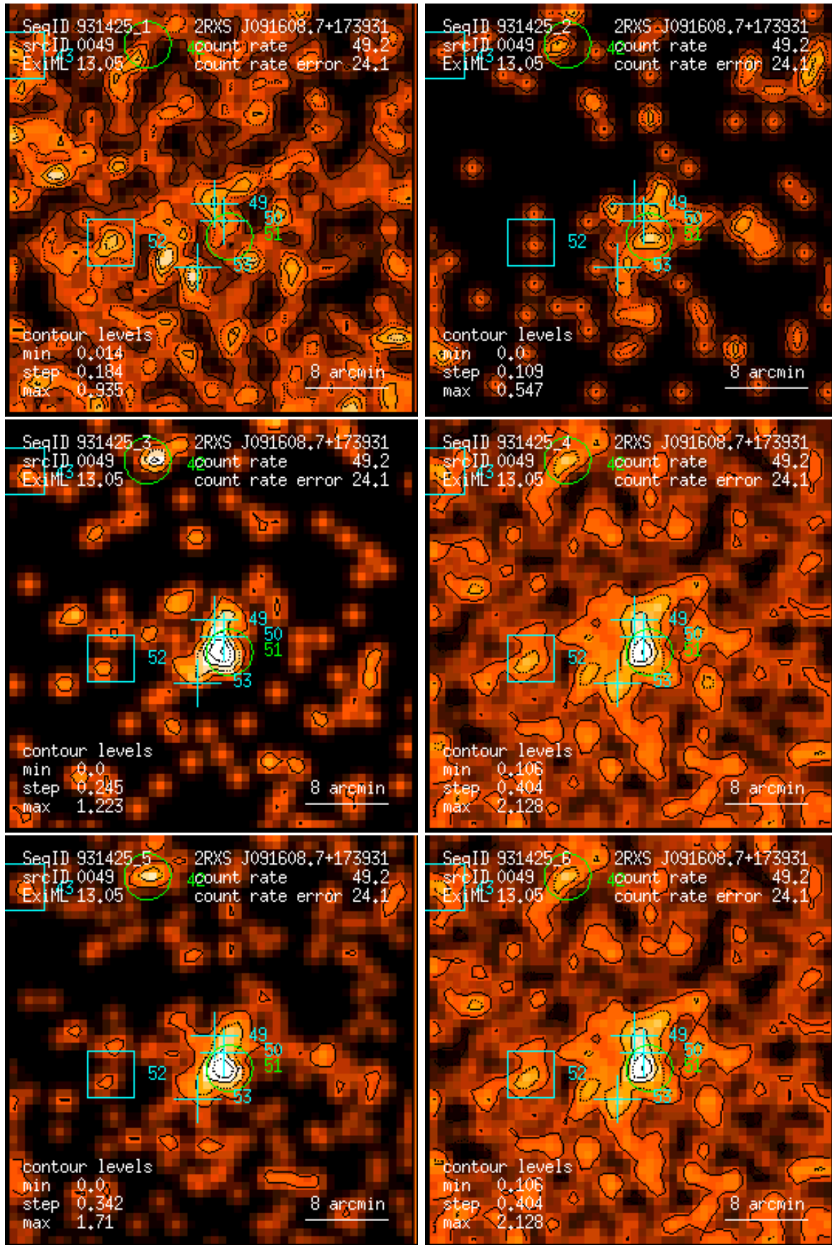
Figure 49: RASS 931425: detection 0049: band rate images, Gaussian filter: (1) PSPC channels 11 – 41, (2) 52 – 90, (3) 91 – 201, (4) 11 – 235, (5) 52 – 201, (6) 11 – 201. Broad band rates in counts/ks. Band rate contour levels in counts/ks/arcmin 2 .
