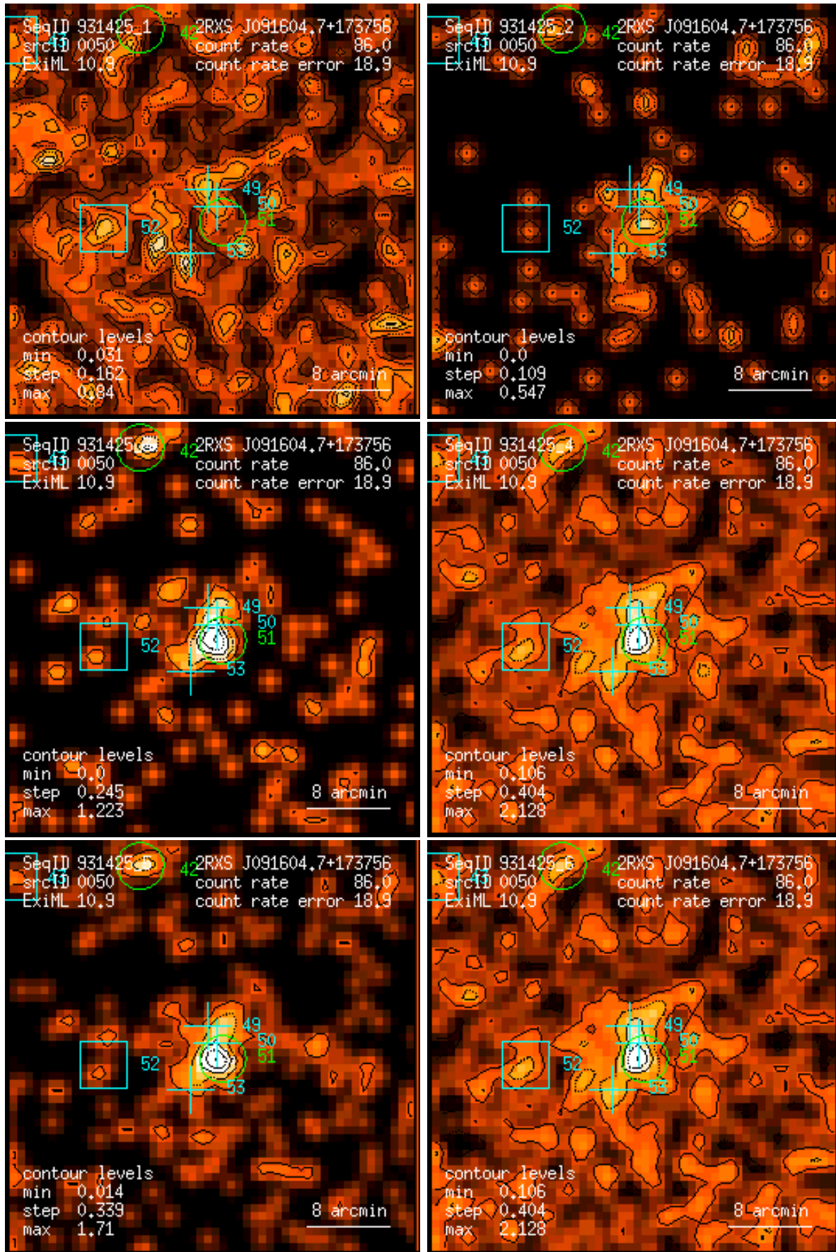
Figure 50: RASS 931425: detection 0050: band rate images, Gaussian filter: (1) PSPC channels 11 – 41, (2) 52 – 90, (3) 91 – 201, (4) 11 – 235, (5) 52 – 201, (6) 11 – 201. Broad band rates in counts/ks. Band rate contour levels in counts/ks/arcmin 2 .
