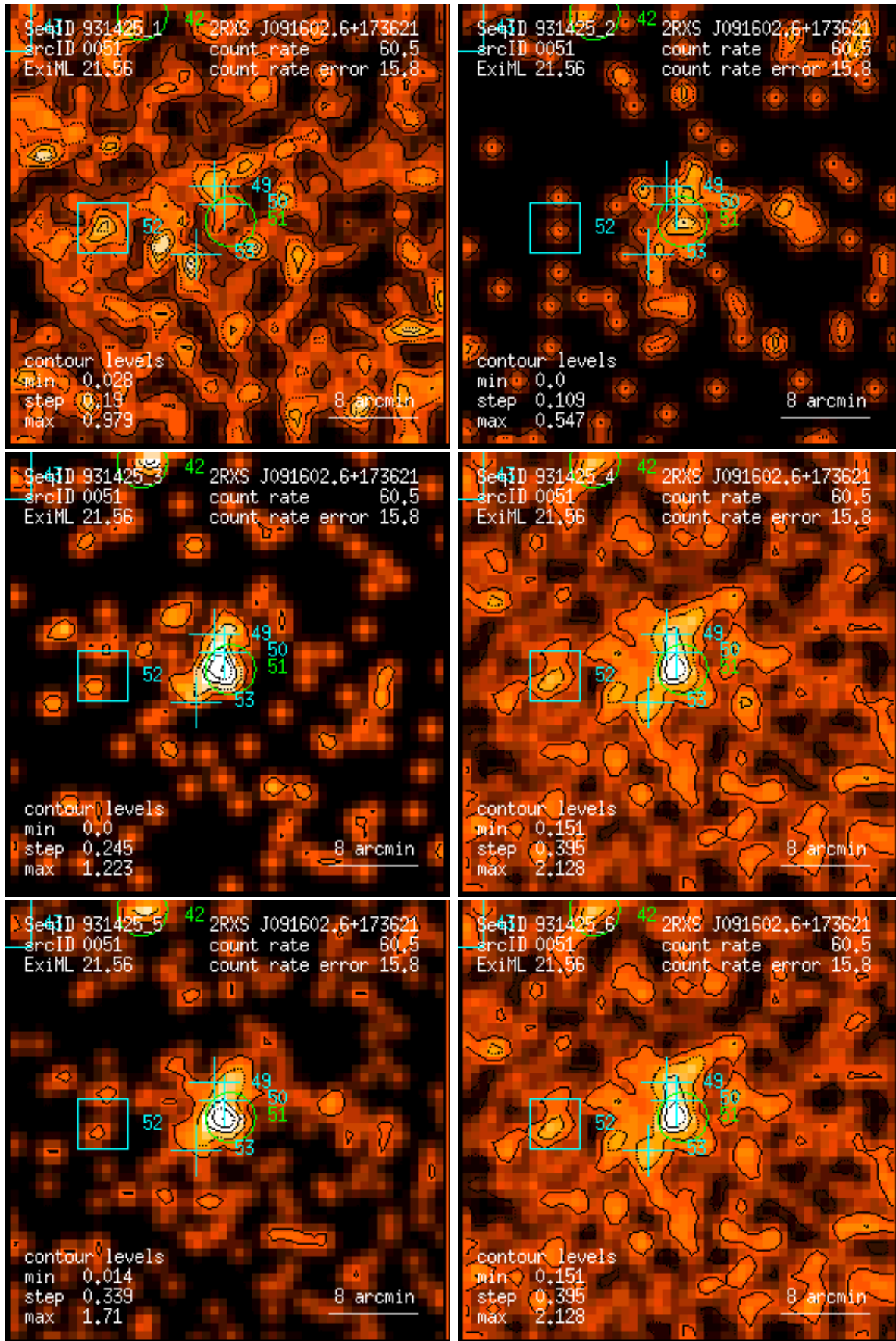
Figure 51: RASS 931425: detection 0051: band rate images, Gaussian filter: (1) PSPC channels 11 – 41, (2) 52 – 90, (3) 91 – 201, (4) 11 – 235, (5) 52 – 201, (6) 11 – 201. Broad band rates in counts/ks. Band rate contour levels in counts/ks/arcmin 2 .
