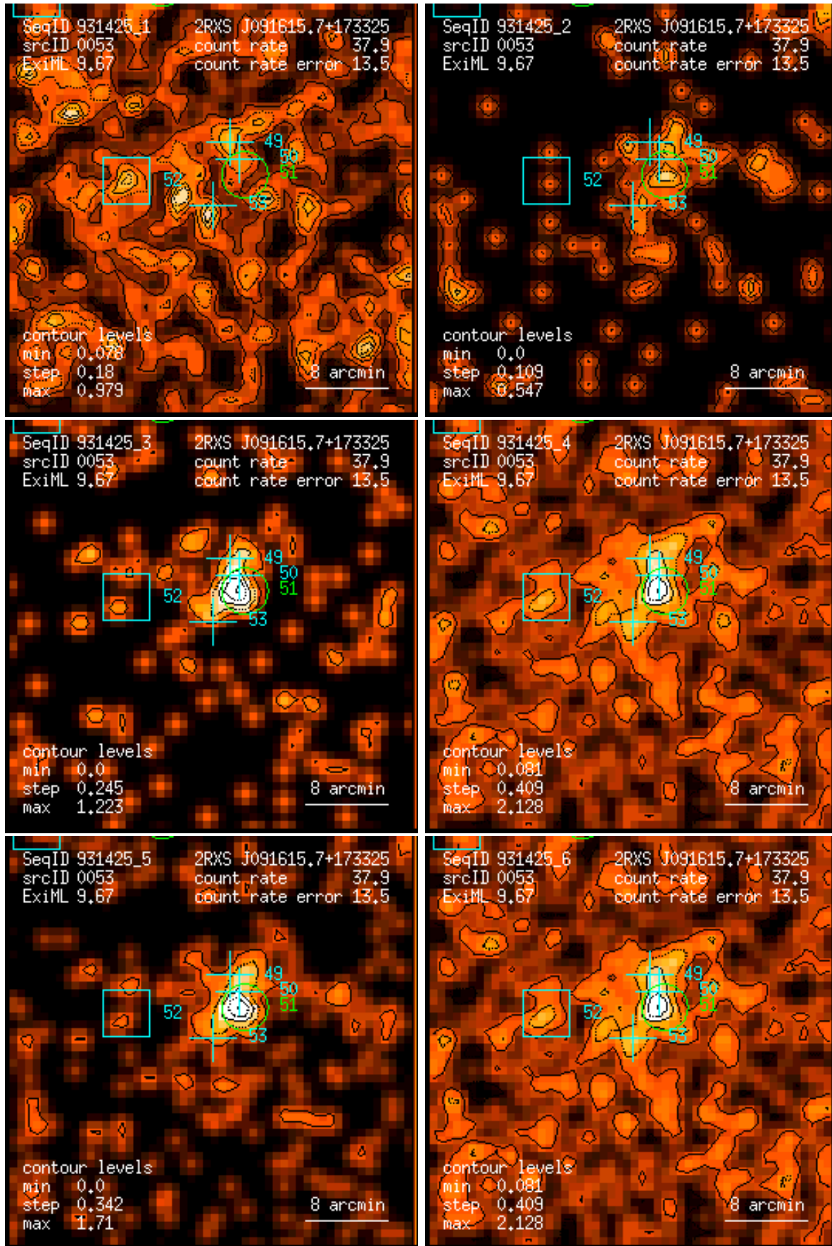
Figure 53: RASS 931425: detection 0053: band rate images, Gaussian filter: (1) PSPC channels 11 – 41, (2) 52 – 90, (3) 91 – 201, (4) 11 – 235, (5) 52 – 201, (6) 11 – 201. Broad band rates in counts/ks. Band rate contour levels in counts/ks/arcmin 2 .
