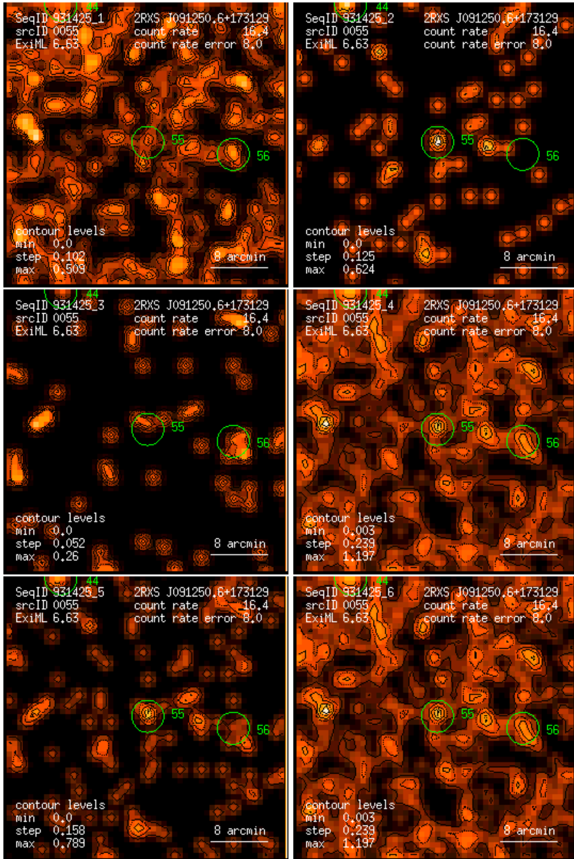
Figure 55: RASS 931425: detection 0055: band rate images, Gaussian filter: (1) PSPC channels 11 – 41, (2) 52 – 90, (3) 91 – 201, (4) 11 – 235, (5) 52 – 201, (6) 11 – 201. Broad band rates in counts/ks. Band rate contour levels in counts/ks/arcmin 2 .
