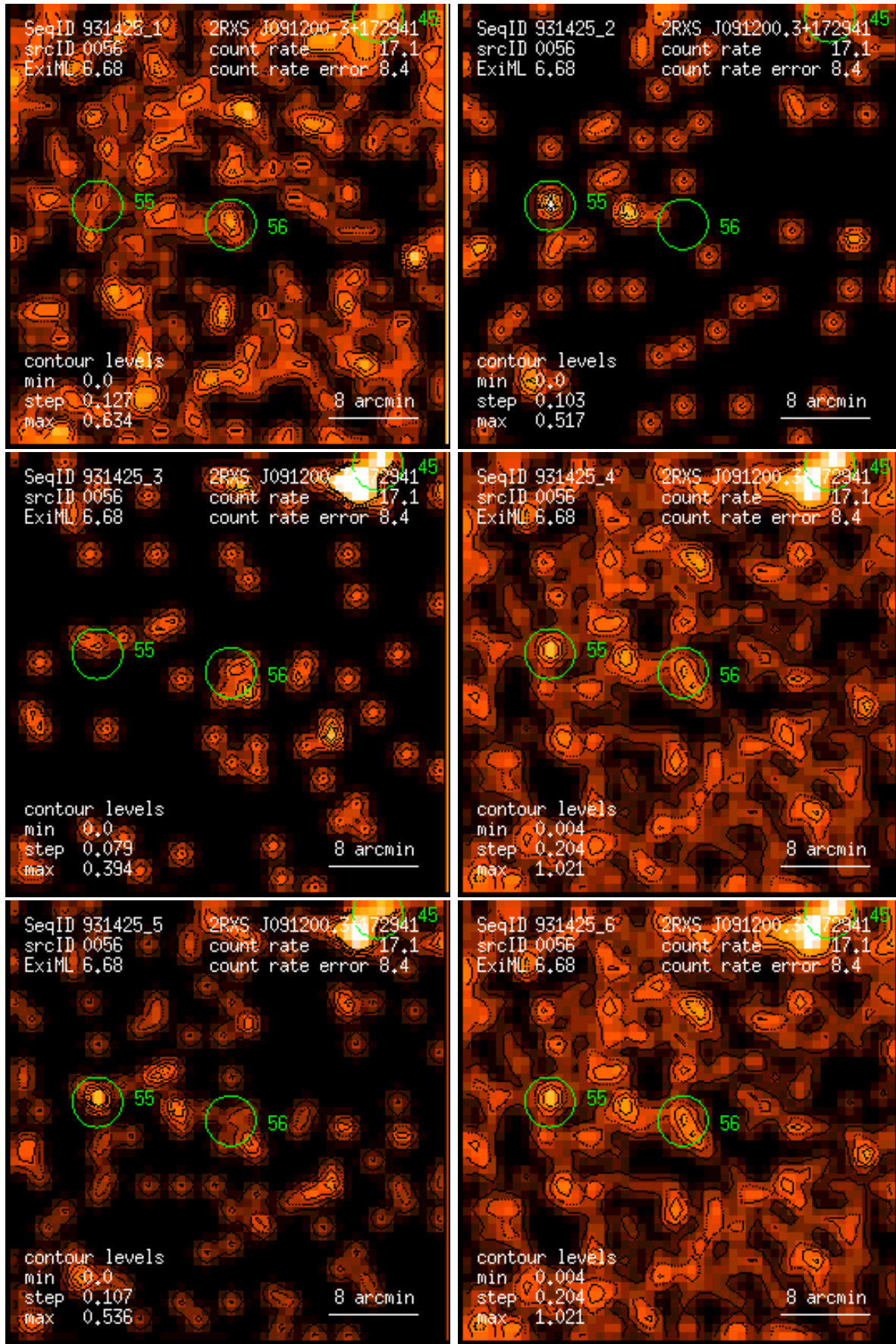
Figure 56: RASS 931425: detection 0056: band rate images, Gaussian filter: (1) PSPC channels 11 – 41, (2) 52 – 90, (3) 91 – 201, (4) 11 – 235, (5) 52 – 201, (6) 11 – 201. Broad band rates in counts/ks. Band rate contour levels in counts/ks/arcmin 2 .
