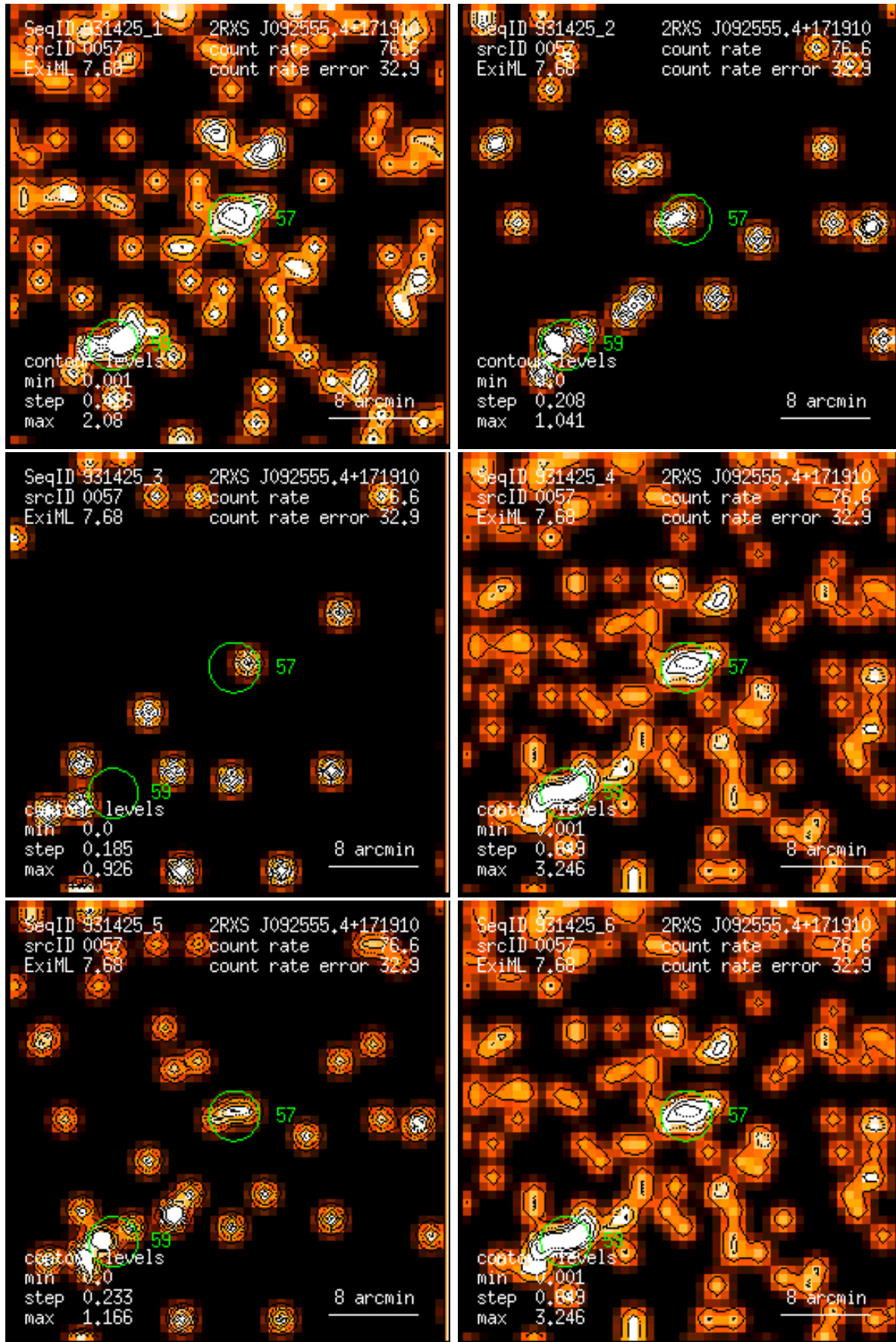
Figure 57: RASS 931425: detection 0057: band rate images, Gaussian filter: (1) PSPC channels 11 – 41, (2) 52 – 90, (3) 91 – 201, (4) 11 – 235, (5) 52 – 201, (6) 11 – 201. Broad band rates in counts/ks. Band rate contour levels in counts/ks/arcmin 2 .
