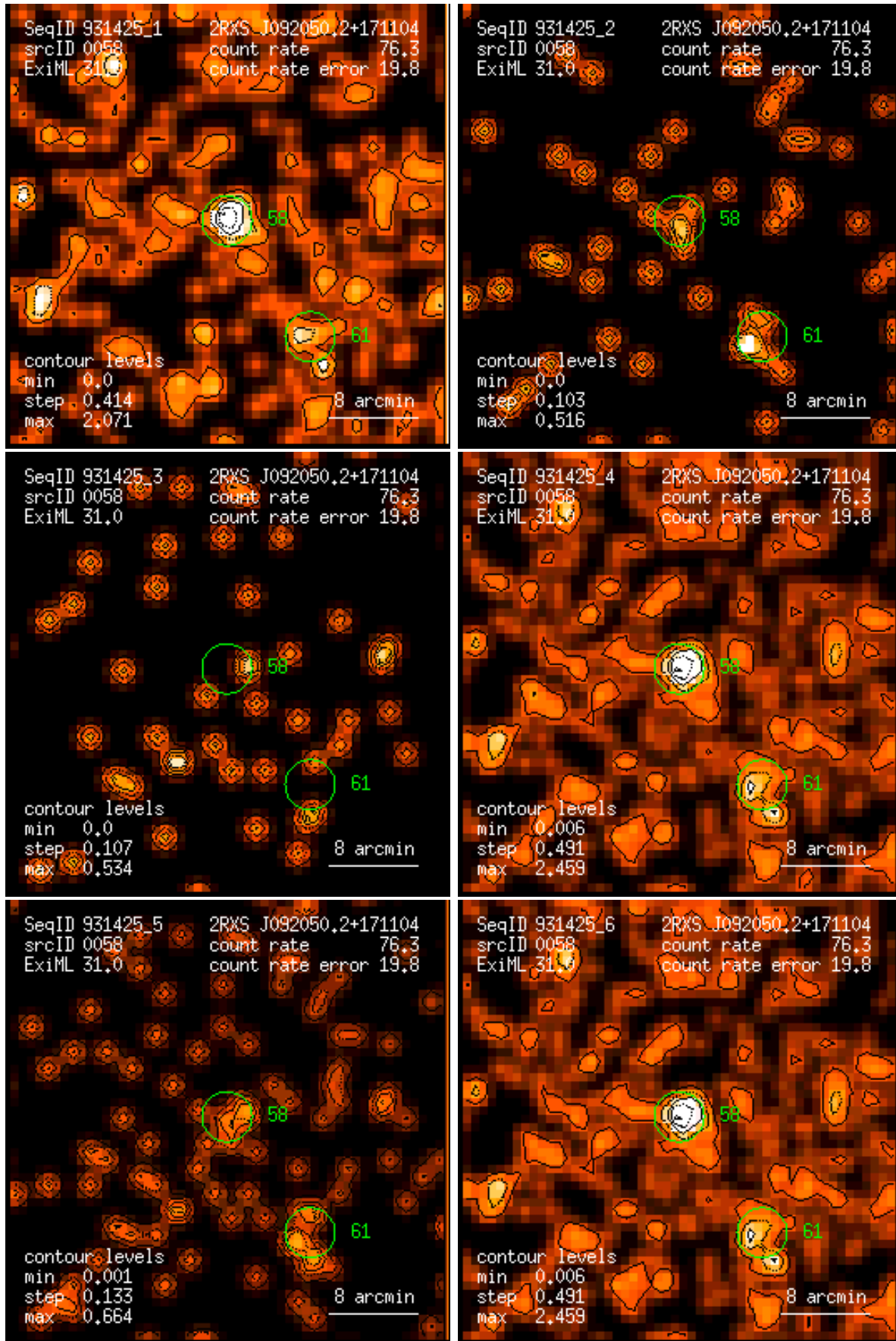
Figure 58: RASS 931425: detection 0058: band rate images, Gaussian filter: (1) PSPC channels 11 – 41, (2) 52 – 90, (3) 91 – 201, (4) 11 – 235, (5) 52 – 201, (6) 11 – 201. Broad band rates in counts/ks. Band rate contour levels in counts/ks/arcmin 2 .
