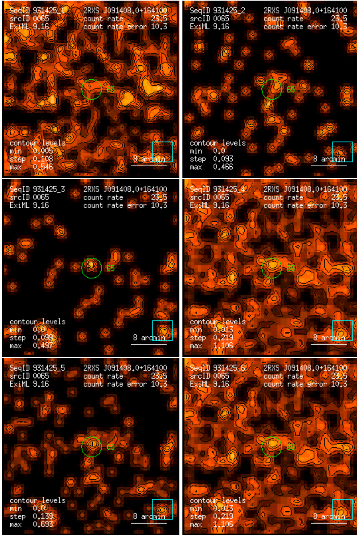
Figure 65: RASS 931425: detection 0065: band rate images, Gaussian filter: (1) PSPC channels 11 – 41, (2) 52 – 90, (3) 91 – 201, (4) 11 – 235, (5) 52 – 201, (6) 11 – 201. Broad band rates in counts/ks. Band rate contour levels in counts/ks/arcmin 2 .
