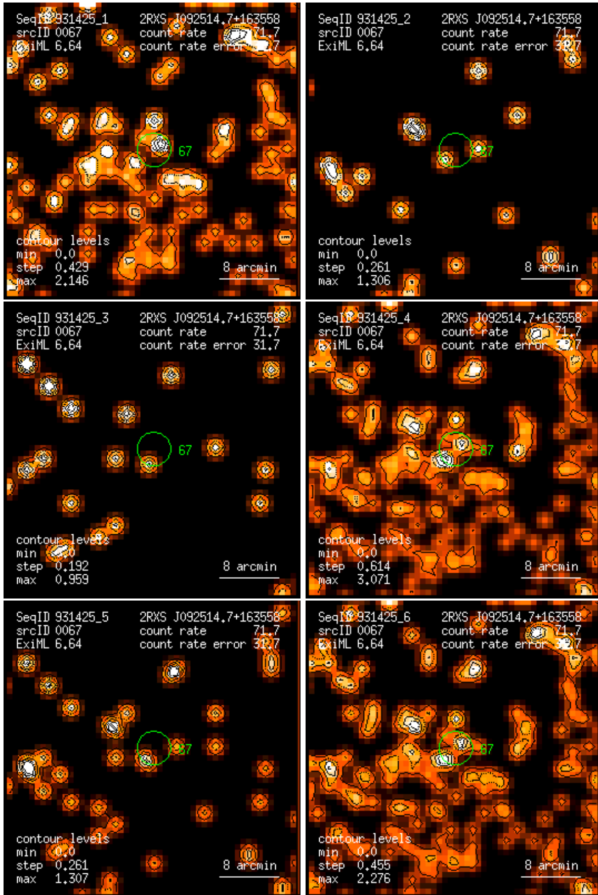
Figure 67: RASS 931425: detection 0067: band rate images, Gaussian filter: (1) PSPC channels 11 – 41, (2) 52 – 90, (3) 91 – 201, (4) 11 – 235, (5) 52 – 201, (6) 11 – 201. Broad band rates in counts/ks. Band rate contour levels in counts/ks/arcmin 2 .
